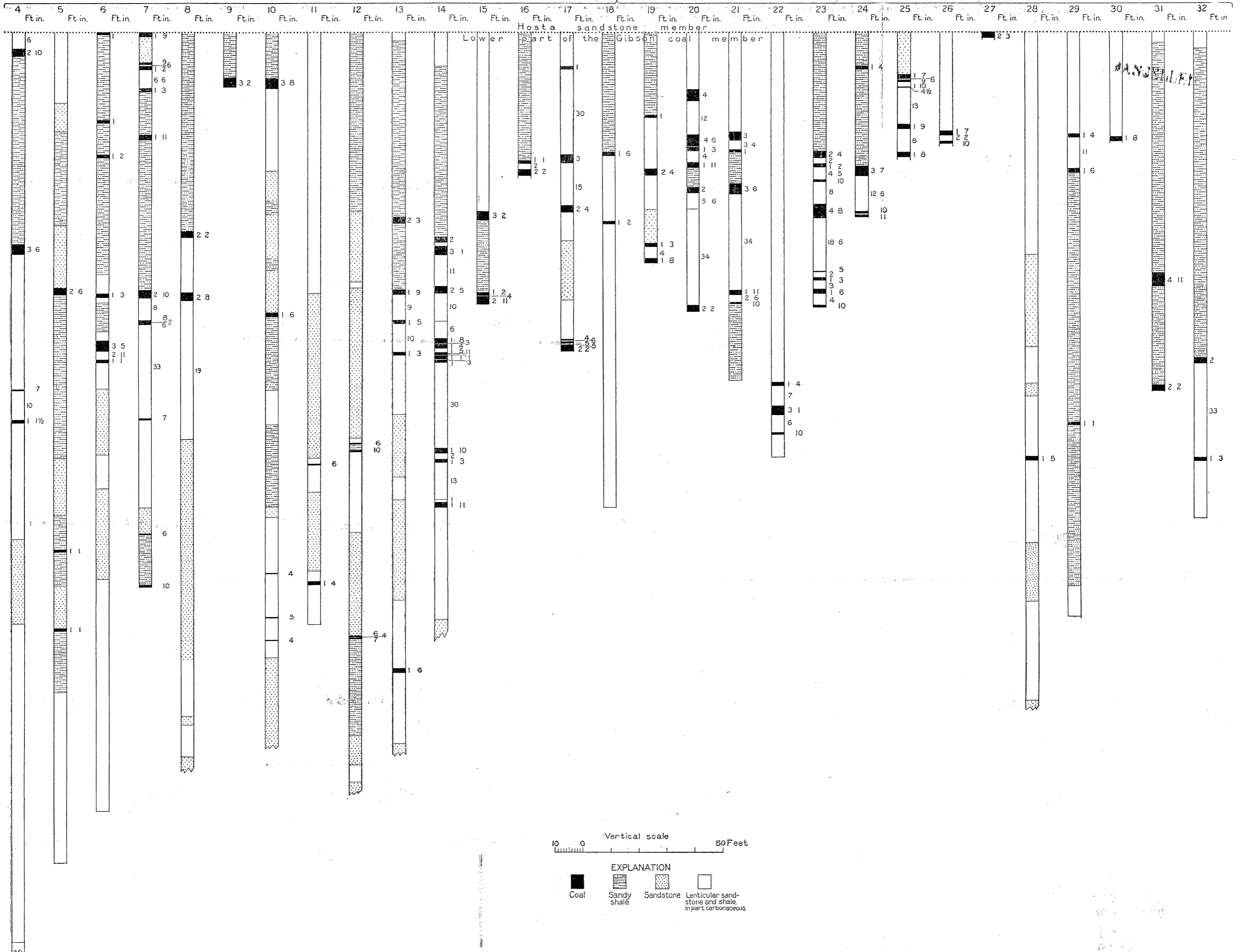
COLUMNAR SECTIONS SHOWING COAL BEDS IN THE LOWER PART OF THE GIBSON COAL MEMBER.
