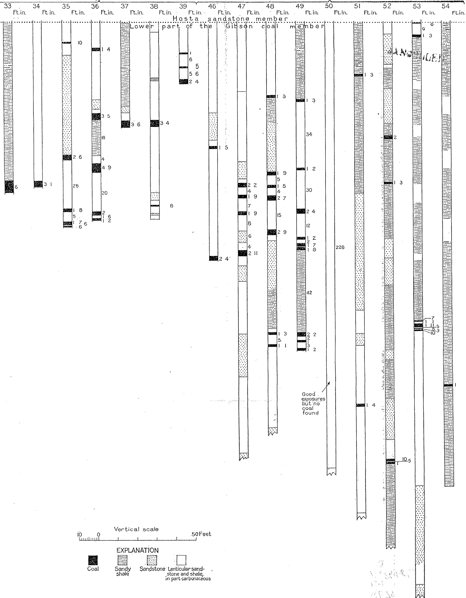
COLUMNAR SECTIONS SHOWING COAL BEDS IN THE LOWER PART OF THE GIBSON COAL MEMBER
