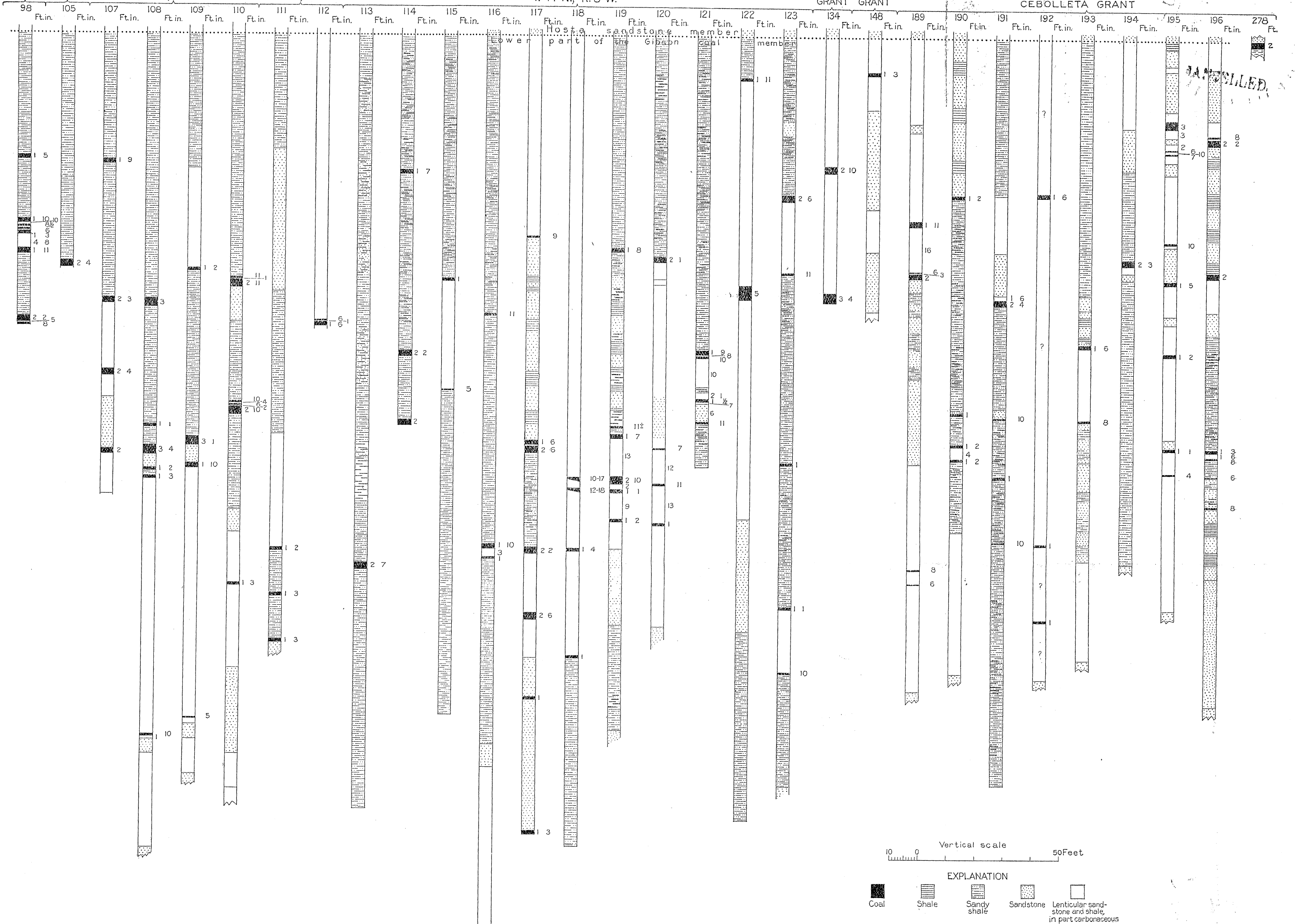
COLUMNAR SECTIONS SHOWING COAL BEDS IN THE LOWER PART OF THE GIBSON COAL MEMBER.
