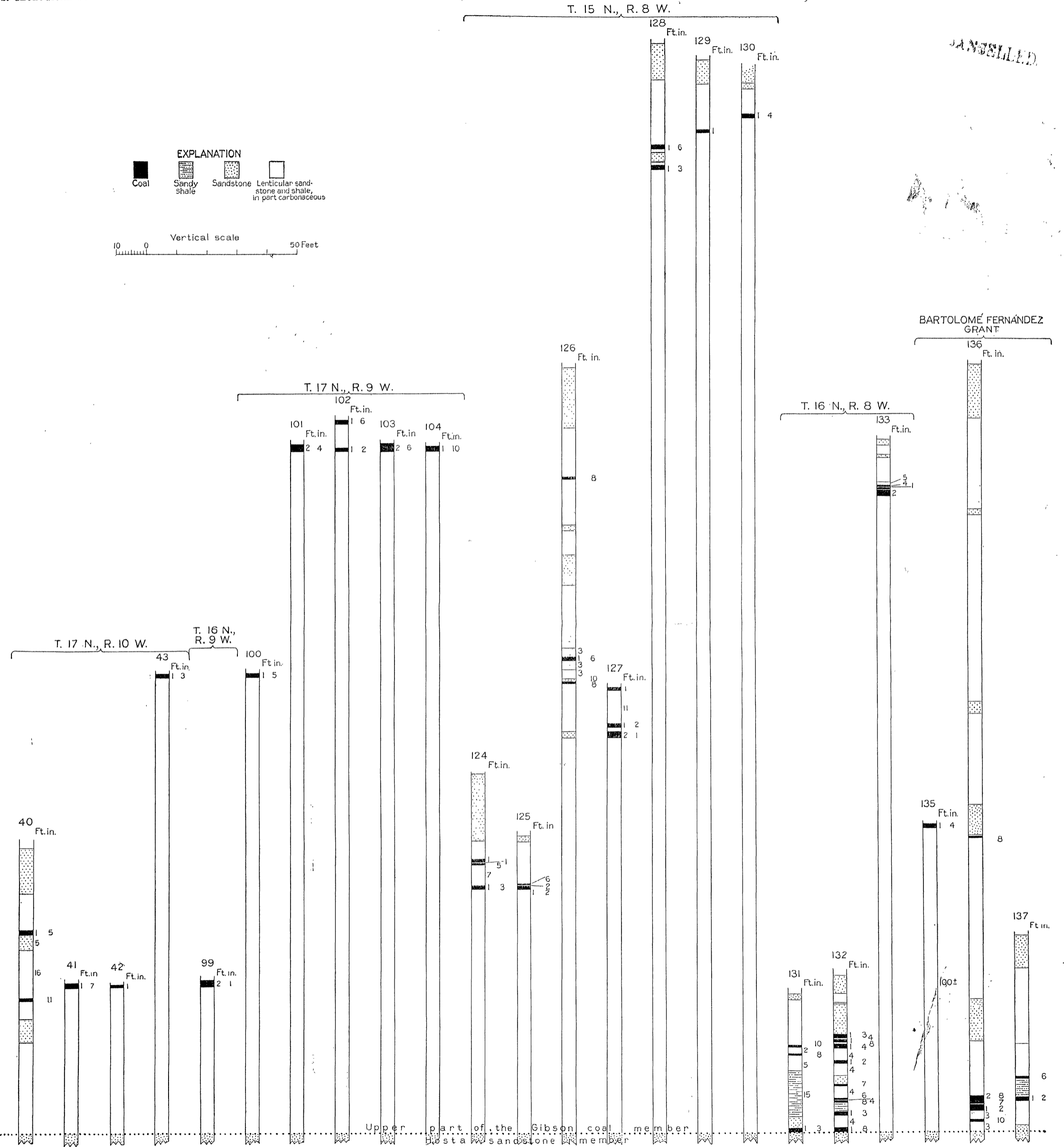
COLUMNAR SECTIONS SHOWING COAL BEDS IN THE UPPER PART OF THE GIBSON COAL MEMBER.
