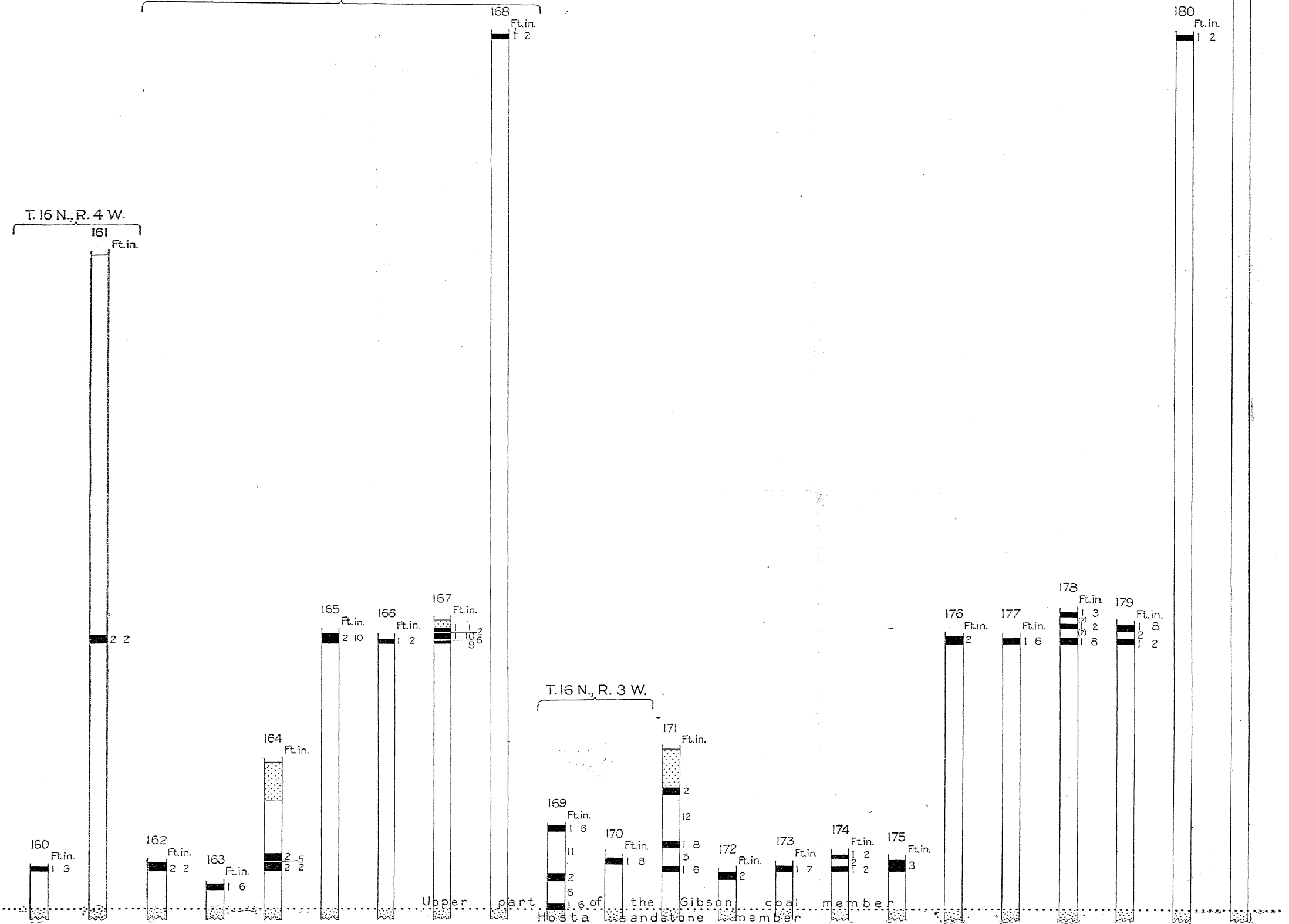
COLUMNAR SECTIONS SHOWING COAL BEDS IN THE UPPER PART OF THE GIBSON COAL MEMBER.
