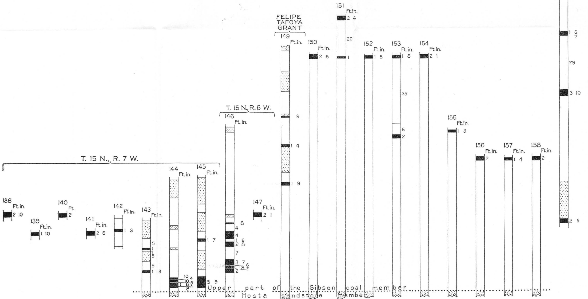
COLUMNAR SECTIONS SHOWING COAL BEDS IN THE UPPER PART OF THE GIBSON COAL MEMBER.
