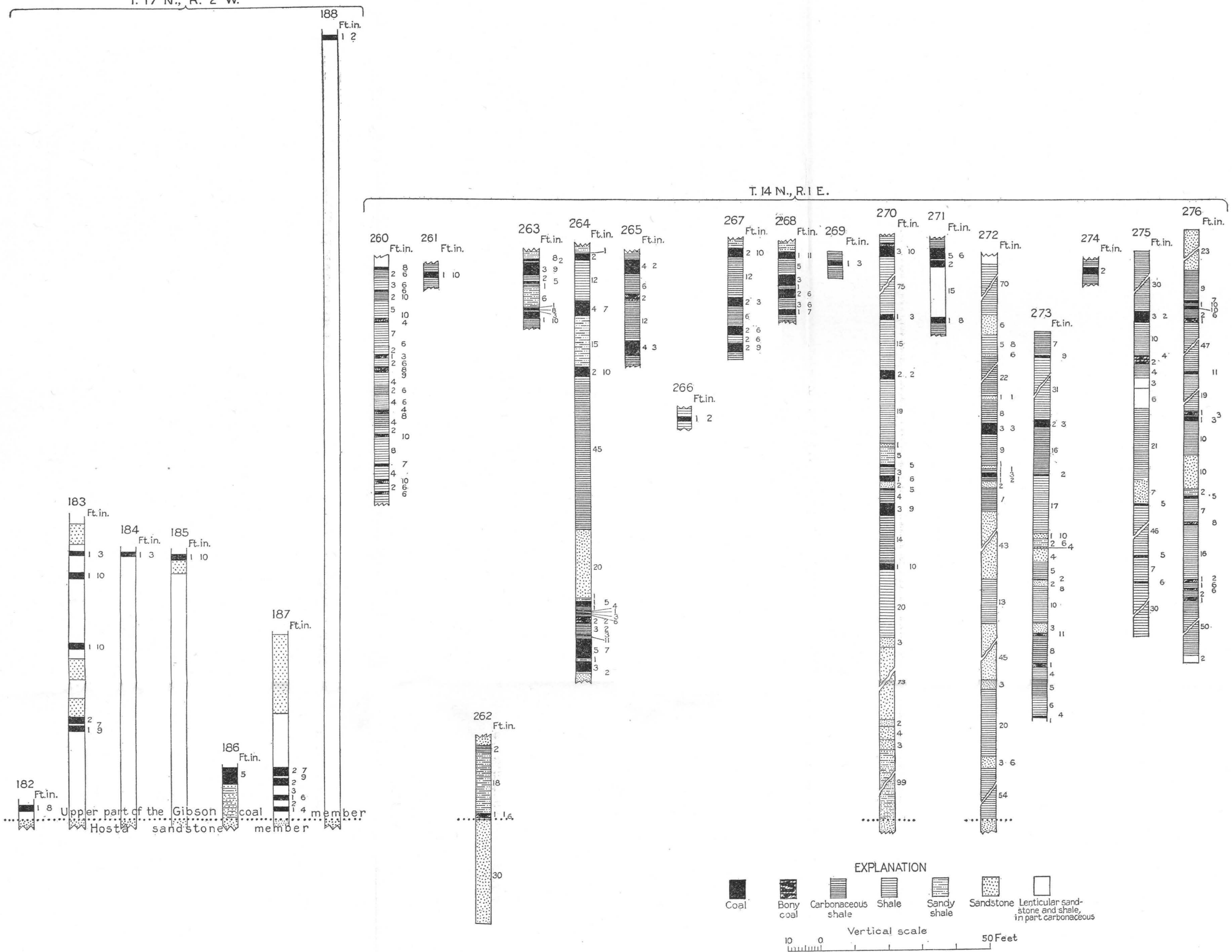
COLUMNAR SECTIONS SHOWING COAL BEDS IN THE UPPER PART OF THE GIBSON COAL MEMBER.
