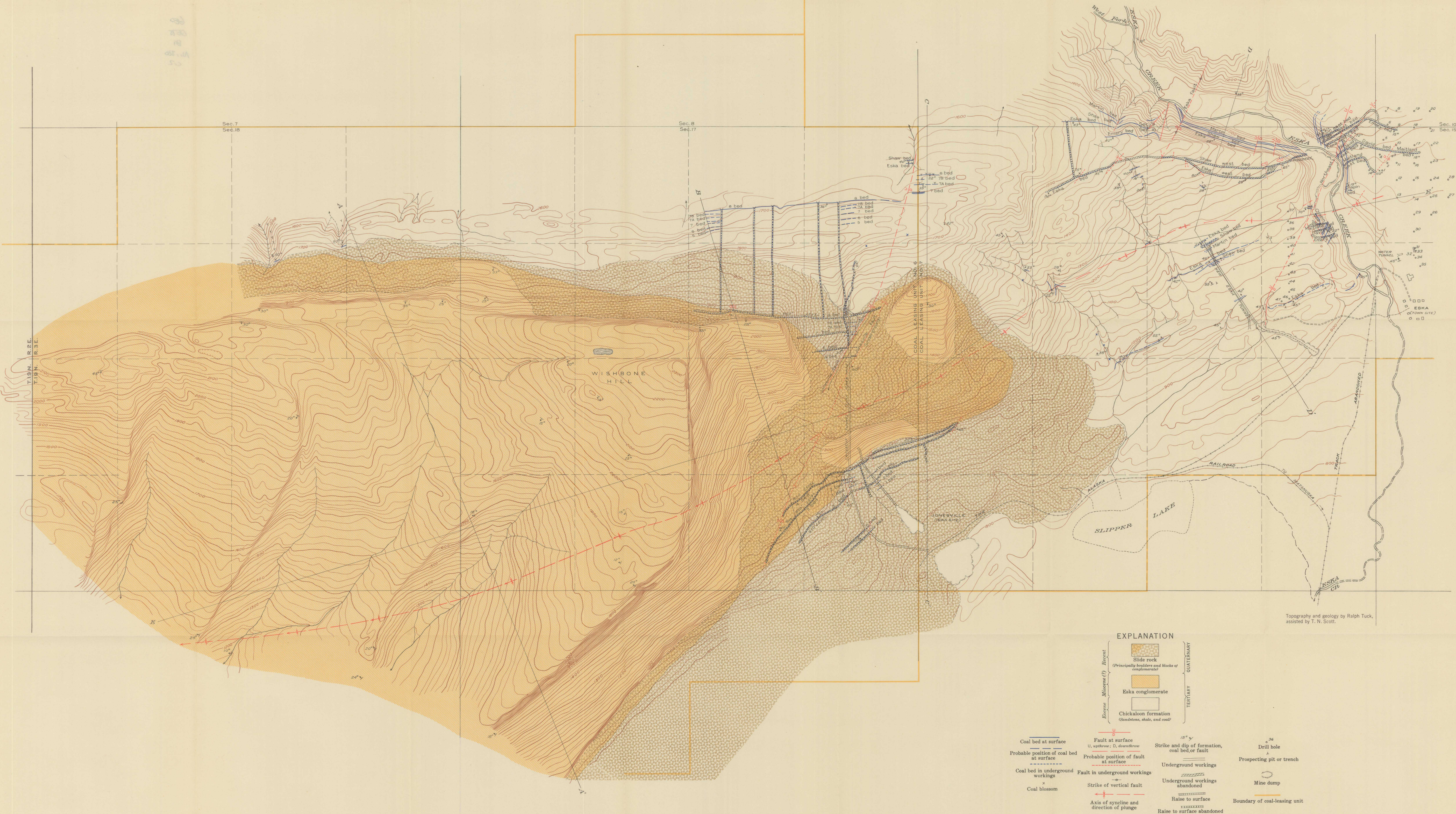
TOPOGRAPHIC AND GEOLOGIC MAP OF THE ESKA CREEK COAL DEPOSITS, MATANUSKA VALLEY, ALASKA
