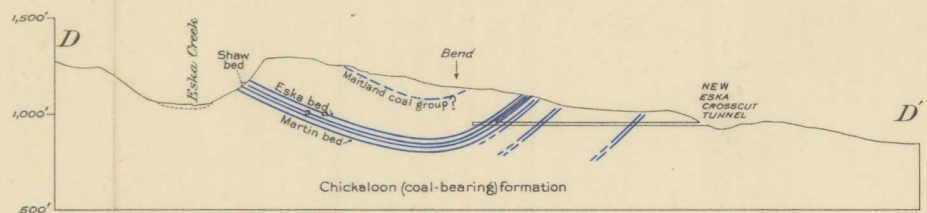
Section along line D-D'
