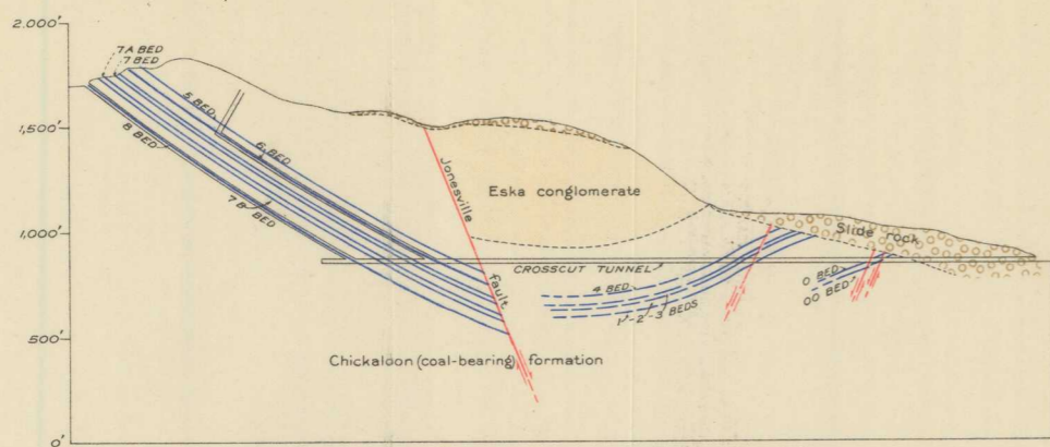
Section through crosscut tunnel, Evan Jones mine
