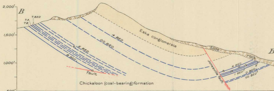
Section along line B-B'
