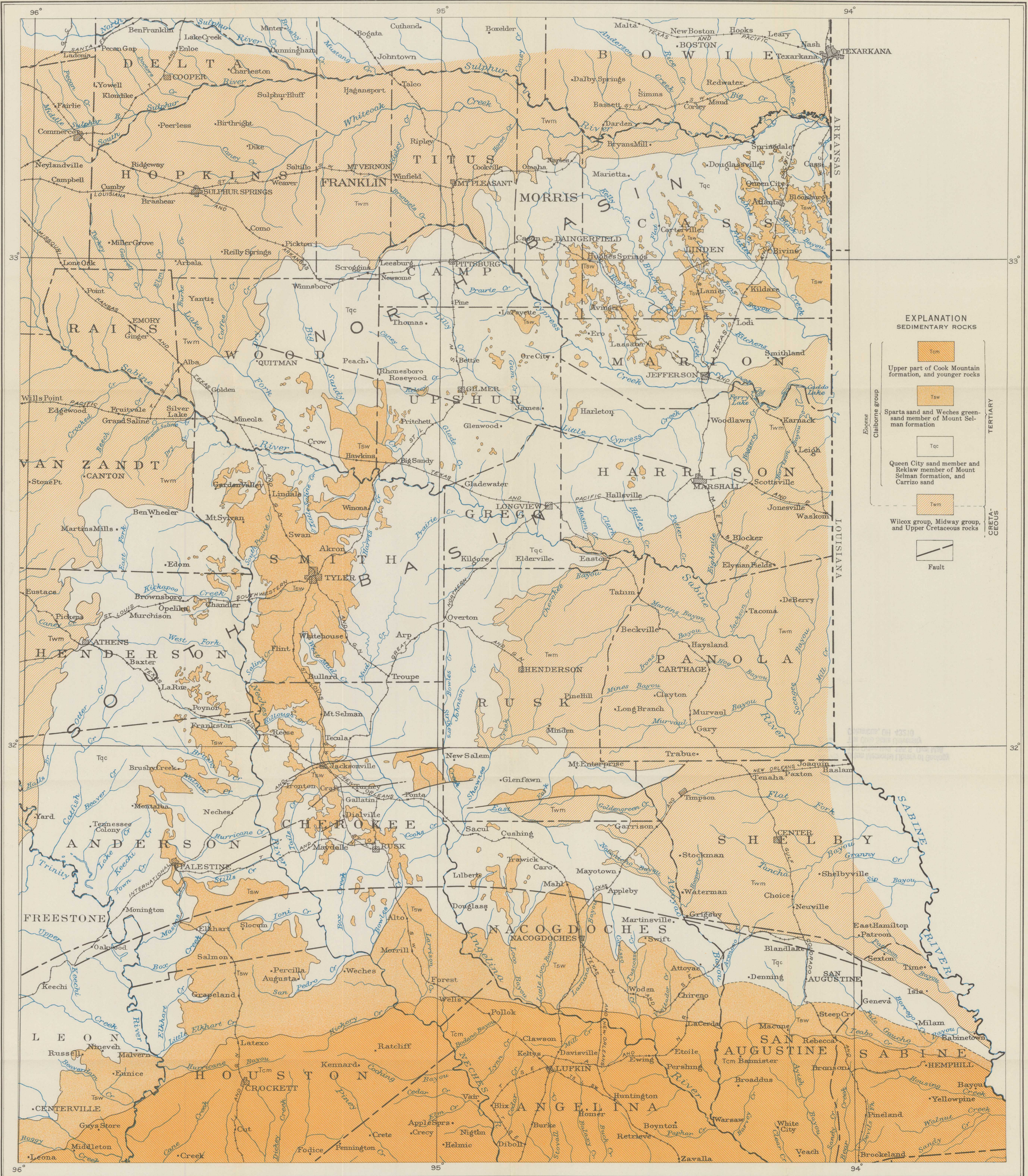
GEOLOGIC MAP SHOWING IRON-BEARING FORMATIONS IN EAST TEXAS
