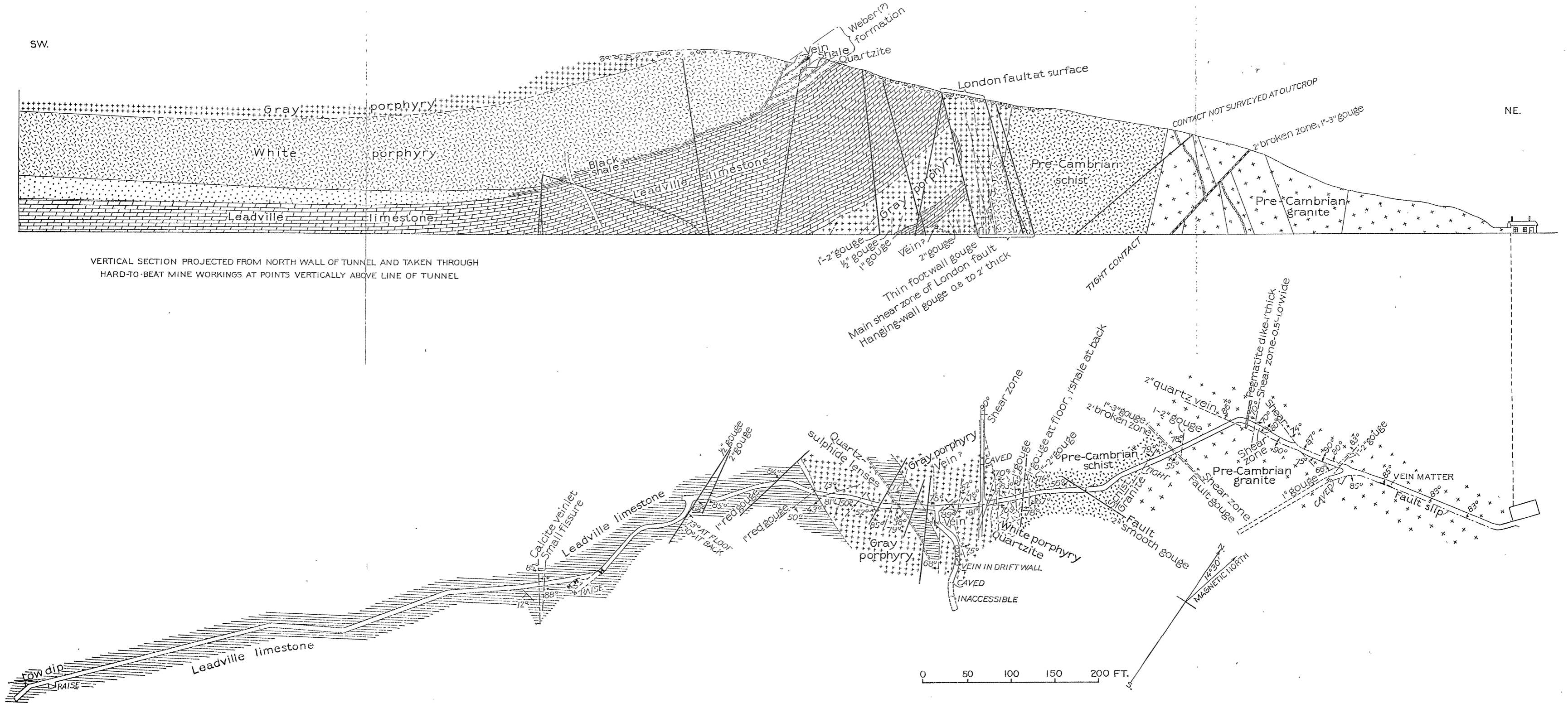
GEOLOGIC MAP AND SECTION OF OLIVER TWIST TUNNEL. East half by F. A. Aicher, west half by Q. D. Singowald.
