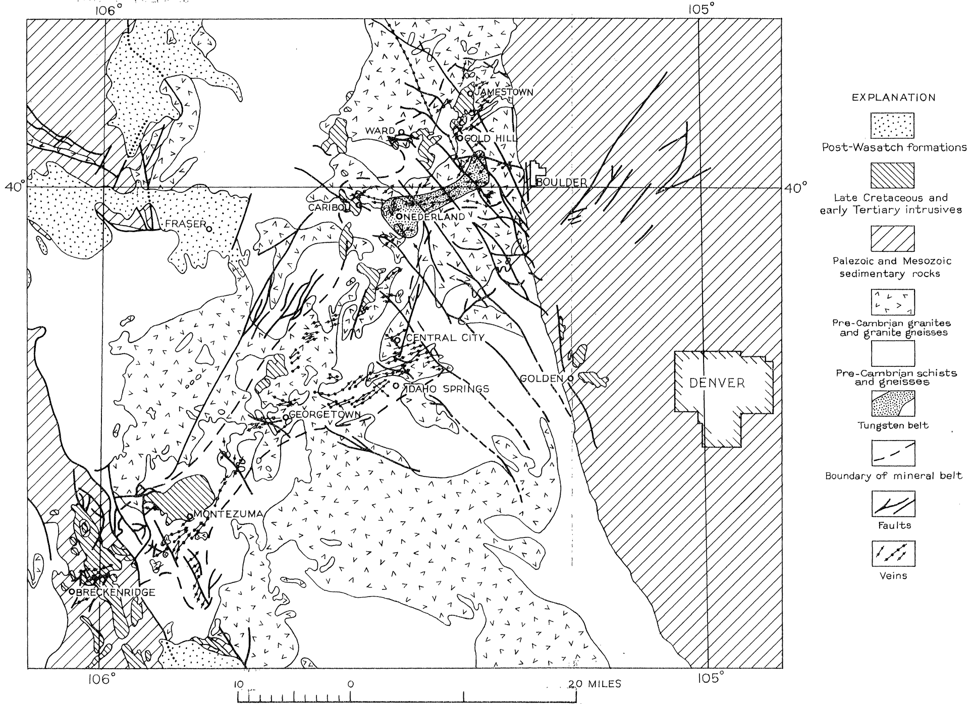
MAP SHOWING THE LOCATION OF THE BOULDER COUNTY TUNGSTEN BELT AND THE GENERAL REGIONAL GEOLOGY
