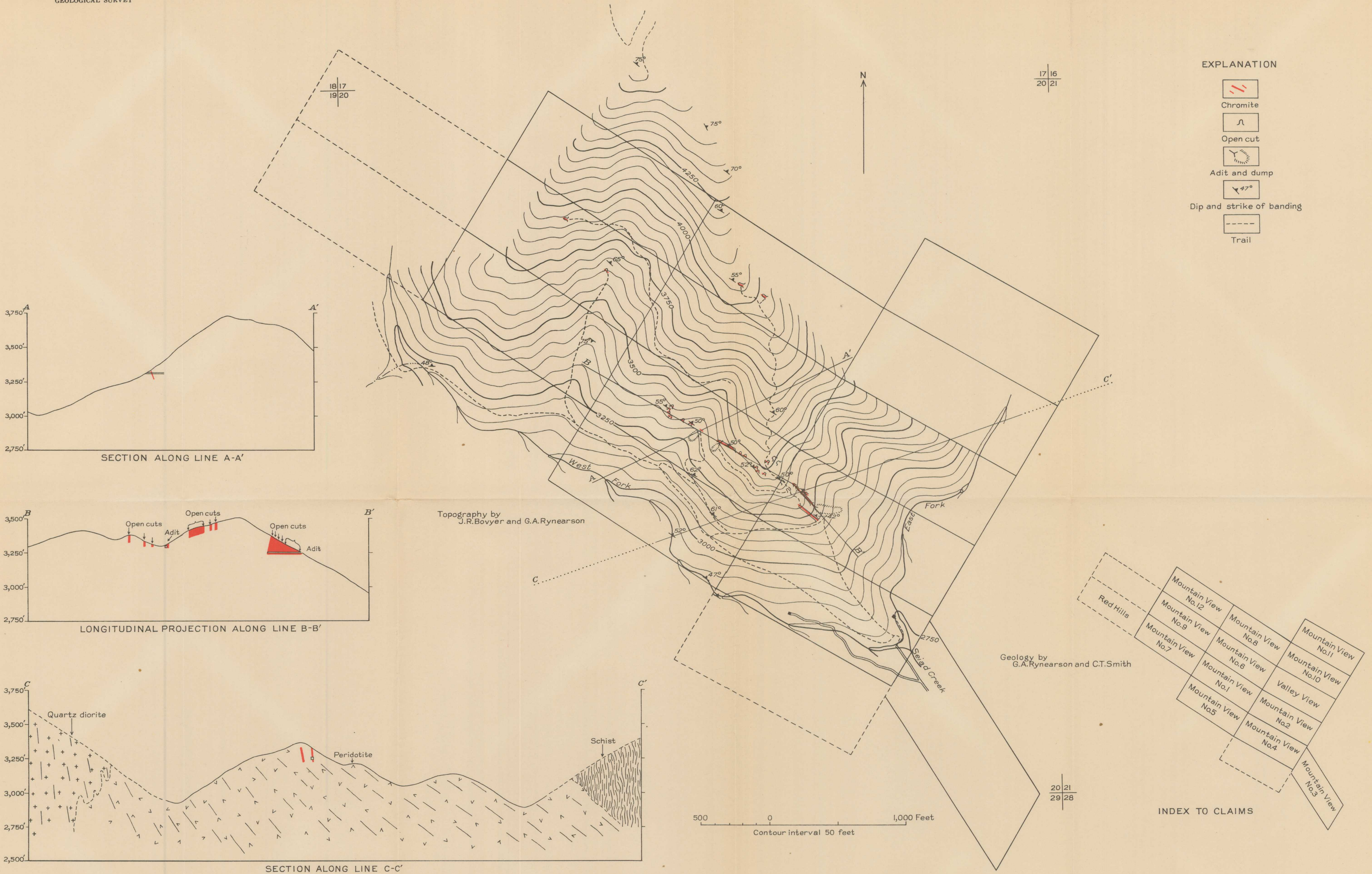
MAP AND SECTIONS OF THE SEIAD CREEK CHROMITE DEPOSIT, SISKIYOU COUNTY, CALIFORNIA
