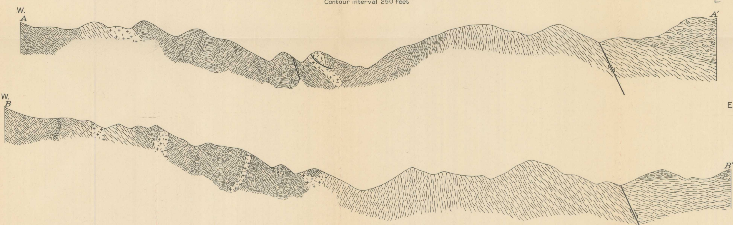
GEOLOGIC MAP AND CROSS SECTIONS OF A PART OF THE AREA BETWEEN WILDROSE AND TUBER CANYONS, PANAMINT RANGE, INYO COUNTY, CALIF.
