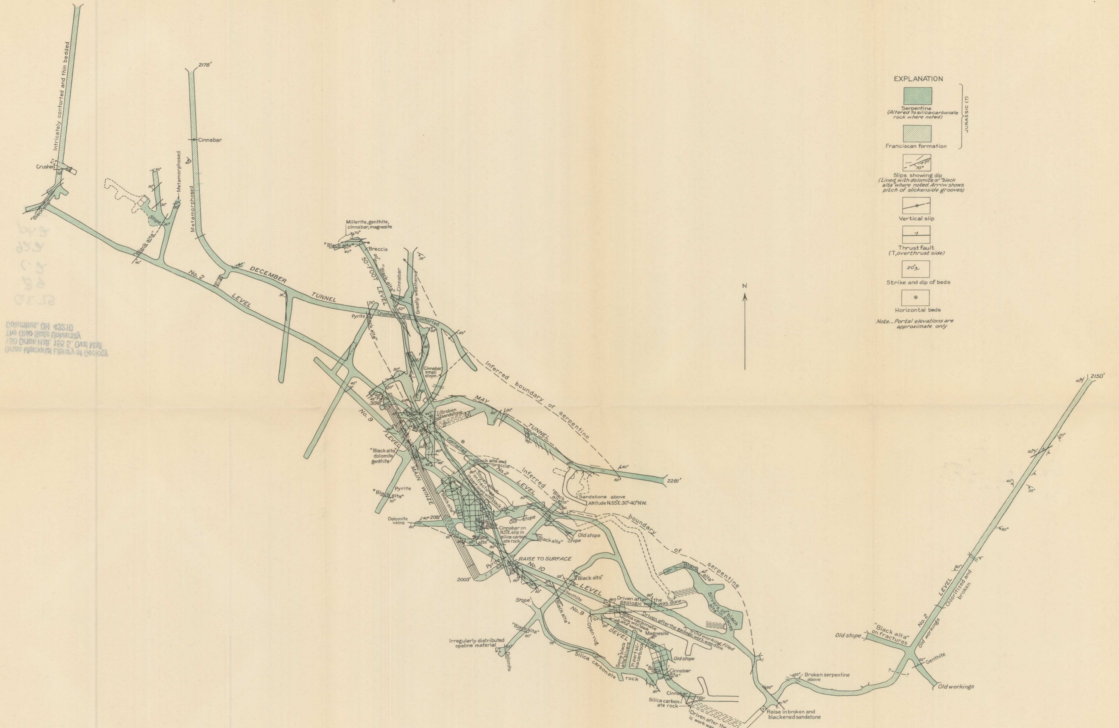
GEOLOGIC MAP OF THE MODERN WORKINGS OF THE GREAT WESTERN MINE, LAKE COUNTY, CALIF.
