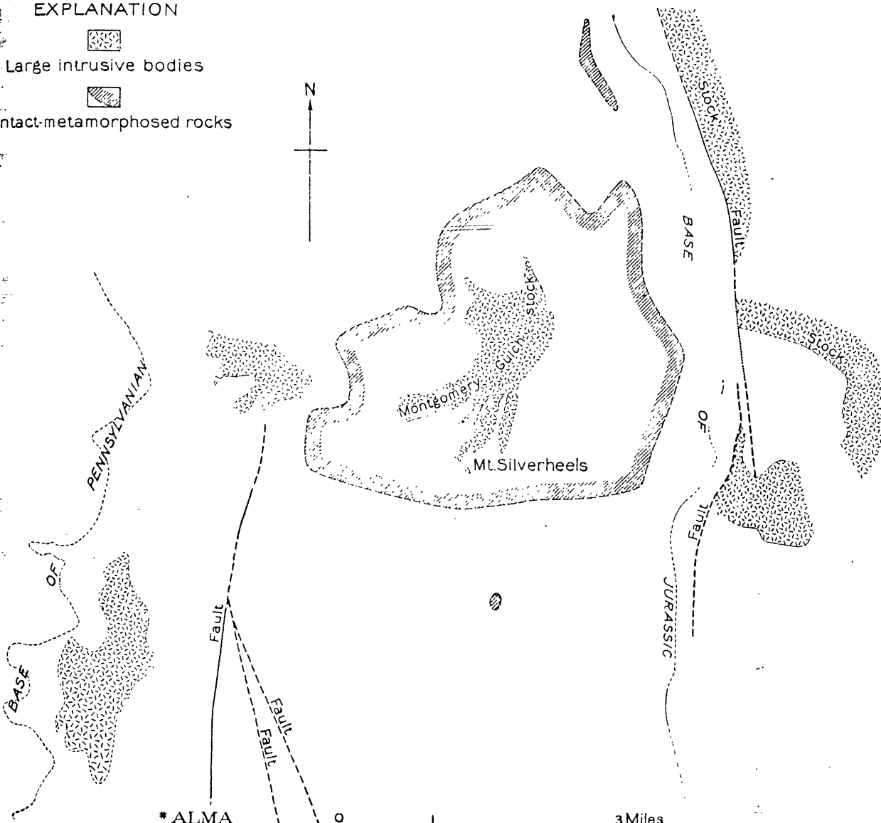
GENERALIZED MAP OF BEAVER-TARRYALL AREA SHOWING
