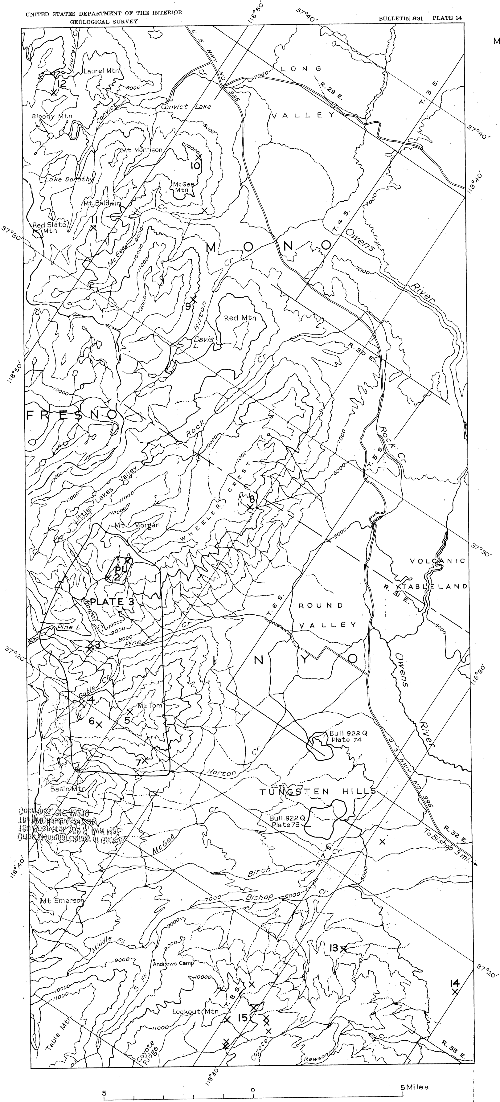
MAP OF PARTS OF THE BISHOP, MT. GODDARD, AND MT. MORRISON QUADRANGLES, INYO COUNTY, CALIFORNIA, SHOWING LOCATION OF THE TUNGSTEN PROPERTIES
