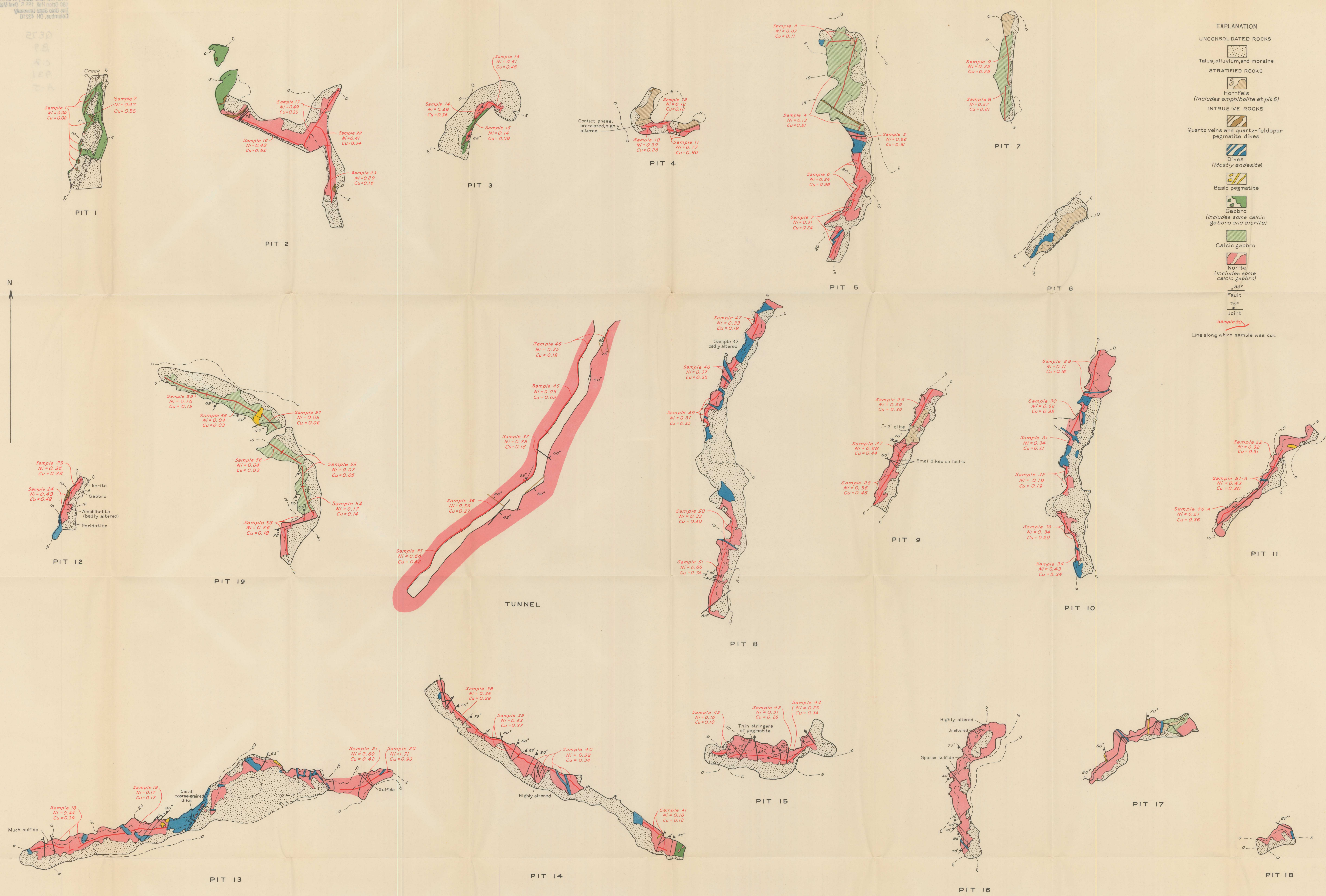
GEOLOGIC MAPS OF PROSPECT PITS AND TUNNEL IN SULFIDE-BEARING BODIES OF BOHEMIA BASIN AND VICINITY, YAKOBI ISLAND, ALASKA
