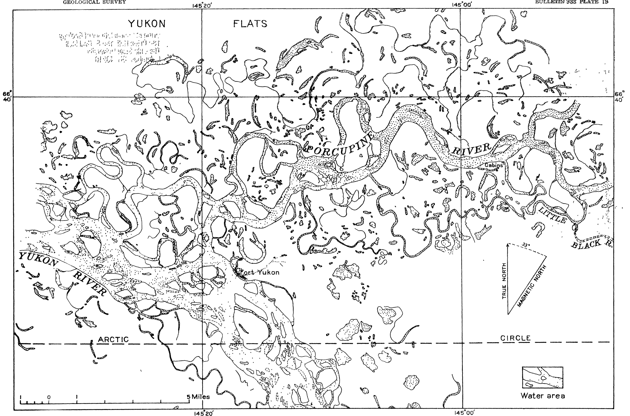
PLANIMETRIC MAP OF LOWER PORCUPINE RIVER, ALASKA
