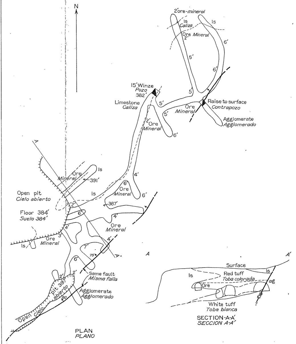
CAFETAL ADIT. TUNEL CAFETAL
