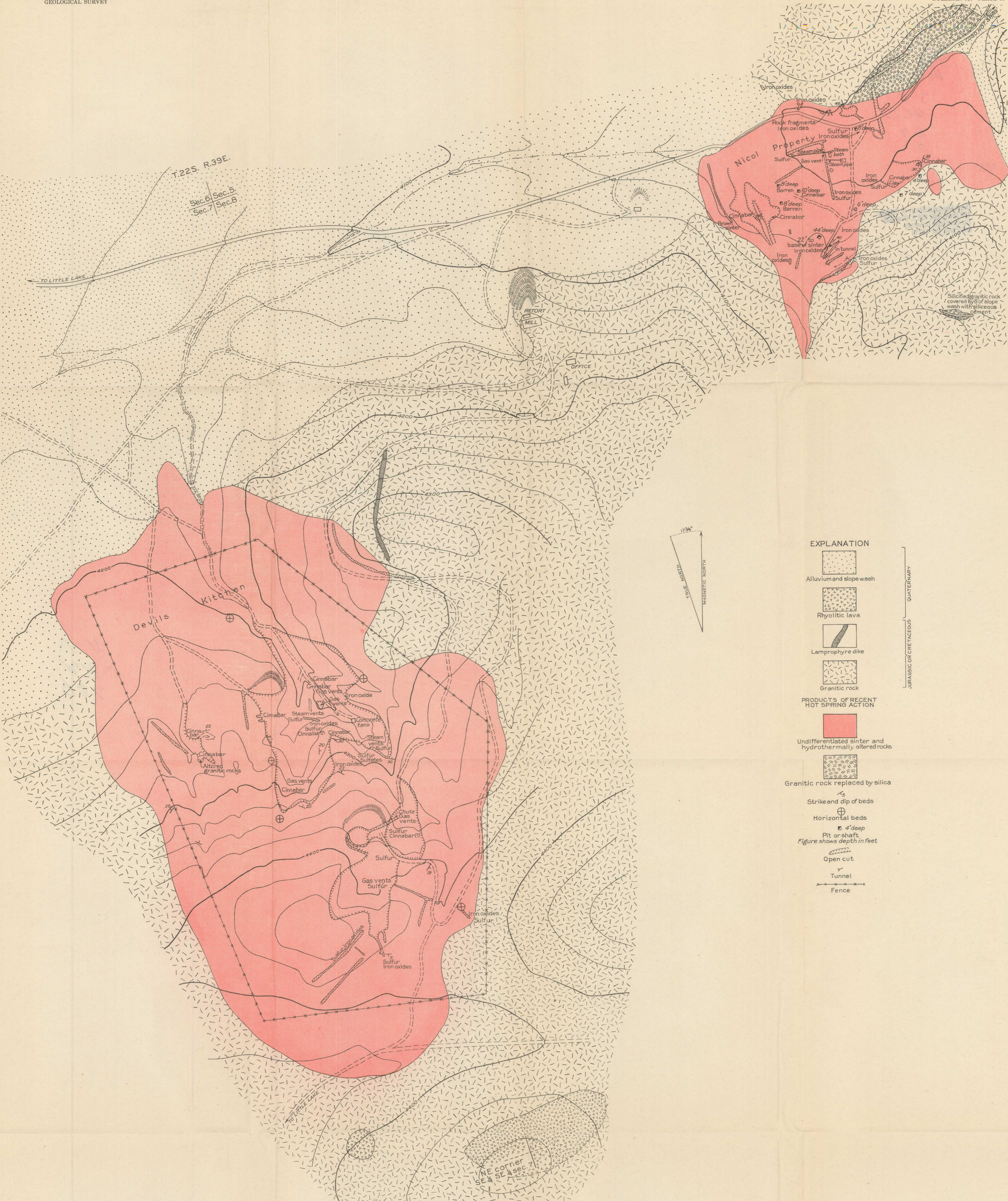
GEOLOGIC AND TOPOGRAPHIC MAP OF THE COSO QUICKSILVER PROPERTY, INYO COUNTY, CALIFORNIA
