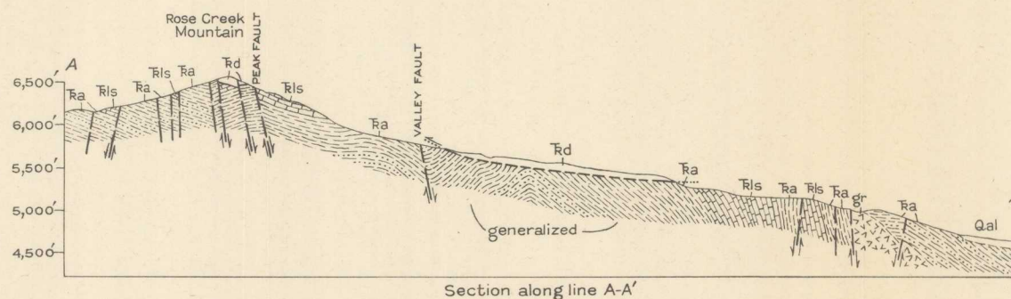
GEOLOGIC MAP AND SECTION OF THE ROSE CREEK AREA, PERSHING COUNTY, NEVADA
