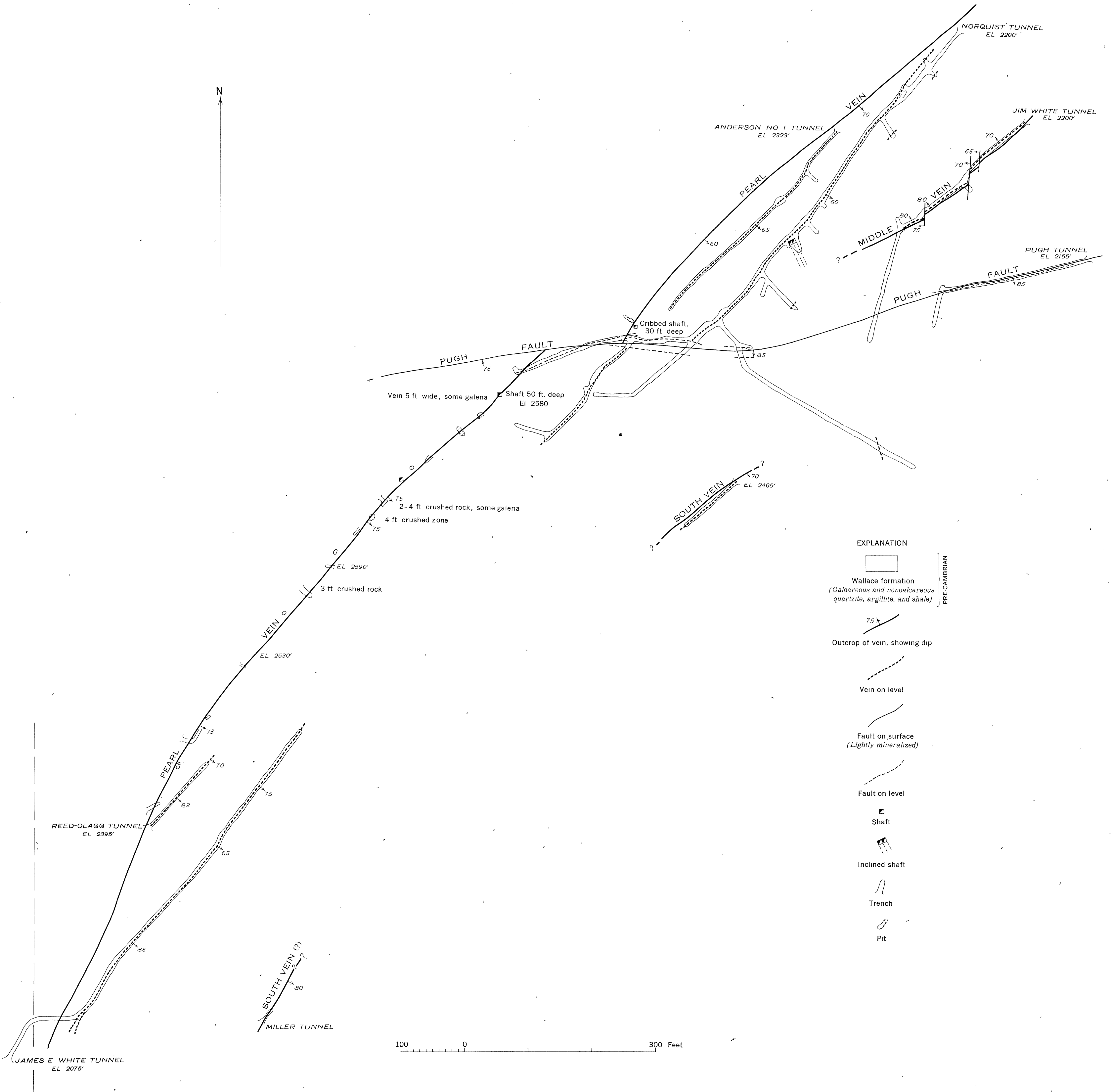
MAP SHOWING FAULT AND VEIN SYSTEMS AT THE WHITEDELFF MINE, BONNER COUNTY, IDAHO
