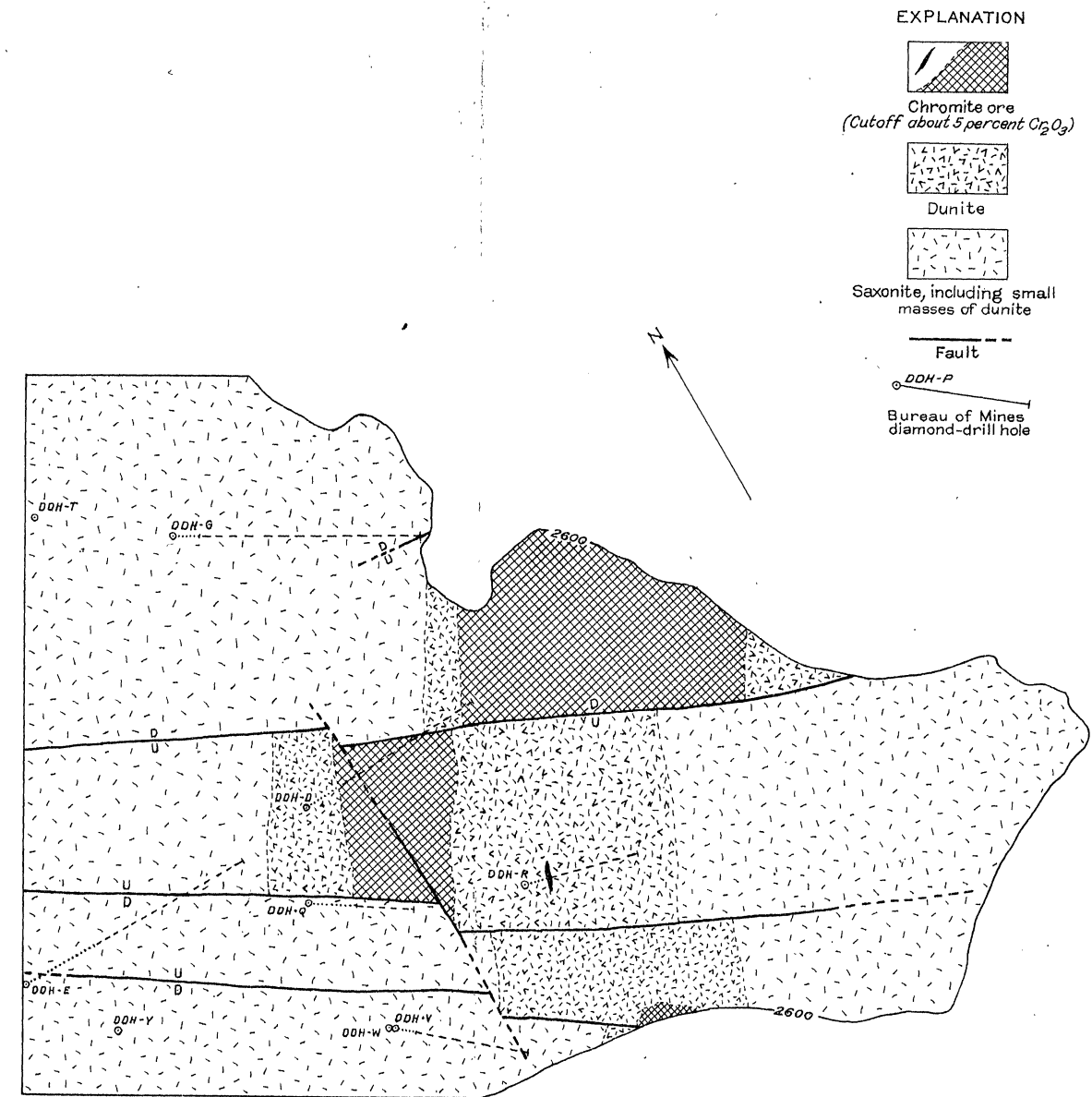
HORIZONTAL SECTION THROUGH 2600 CONTOUR
