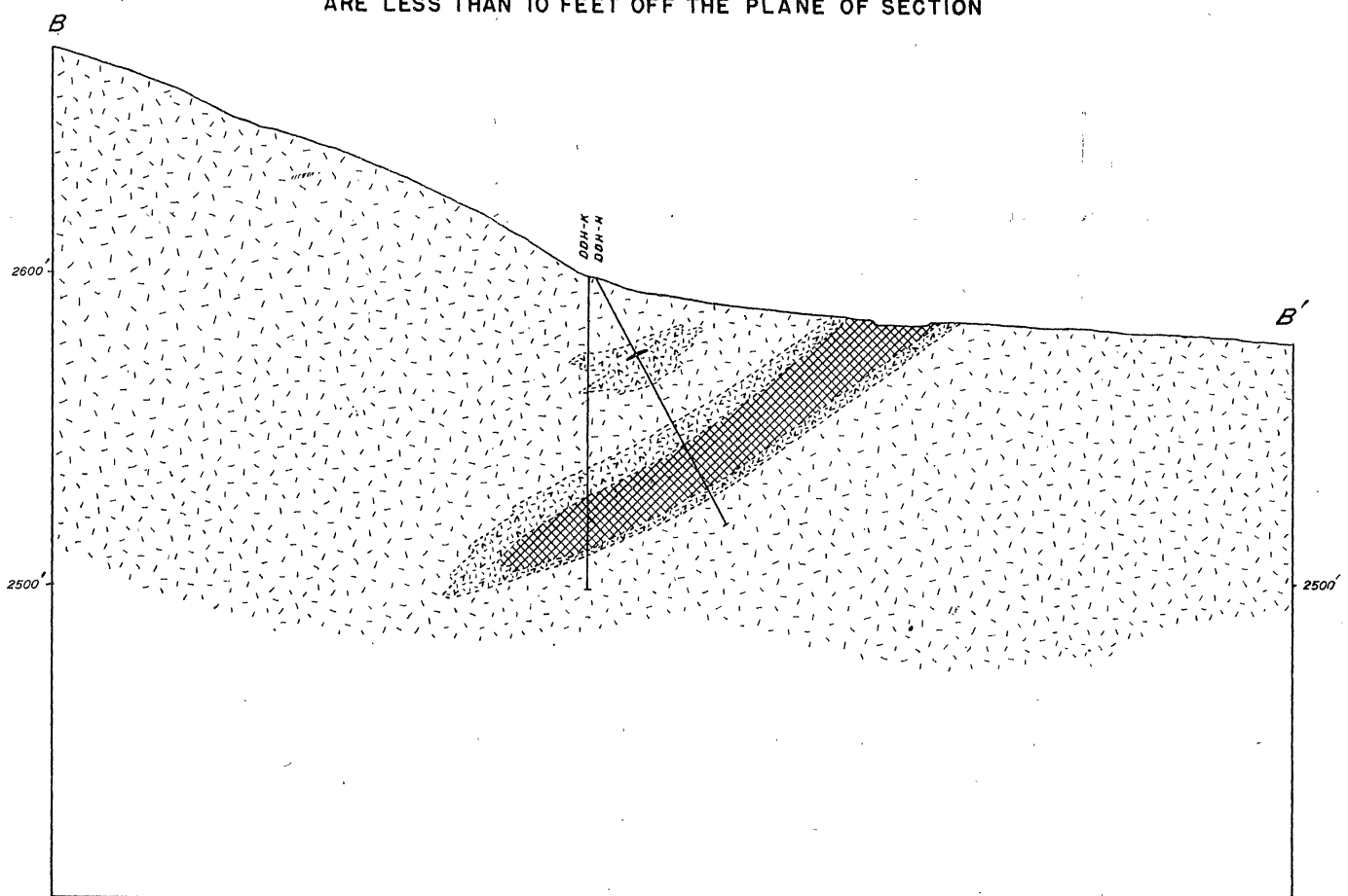
VERTICAL SECTION THROUGH DIAMOND-DRILL HOLES H AND K
