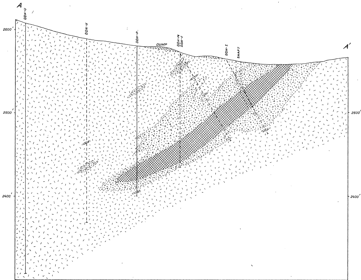
VERTICAL SECTION THROUGH DIAMOND-DRILL HOLES I, J, M, P, X AND U DASHED LINES REPRESENT PROJECTIONS OF DRILL HOLES WHICH ARE LESS THAN 10 FEET OFF THE PLANE OF SECTION
