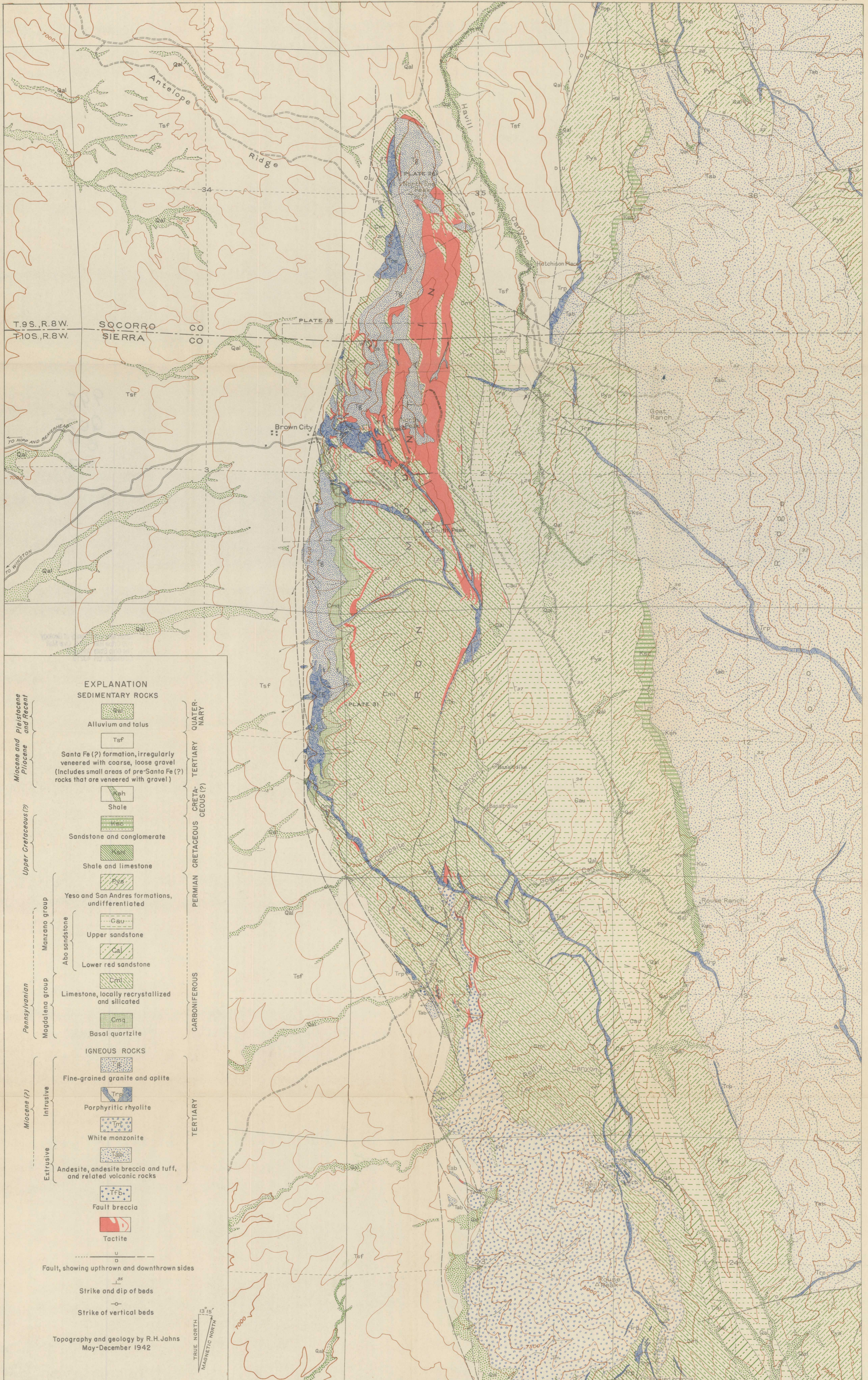
GEOLOGIC MAP OF THE IRON MOUNTAIN DISTRICT, SIERRA AND SOCORRO COUNTIES, NEW MEXICO
