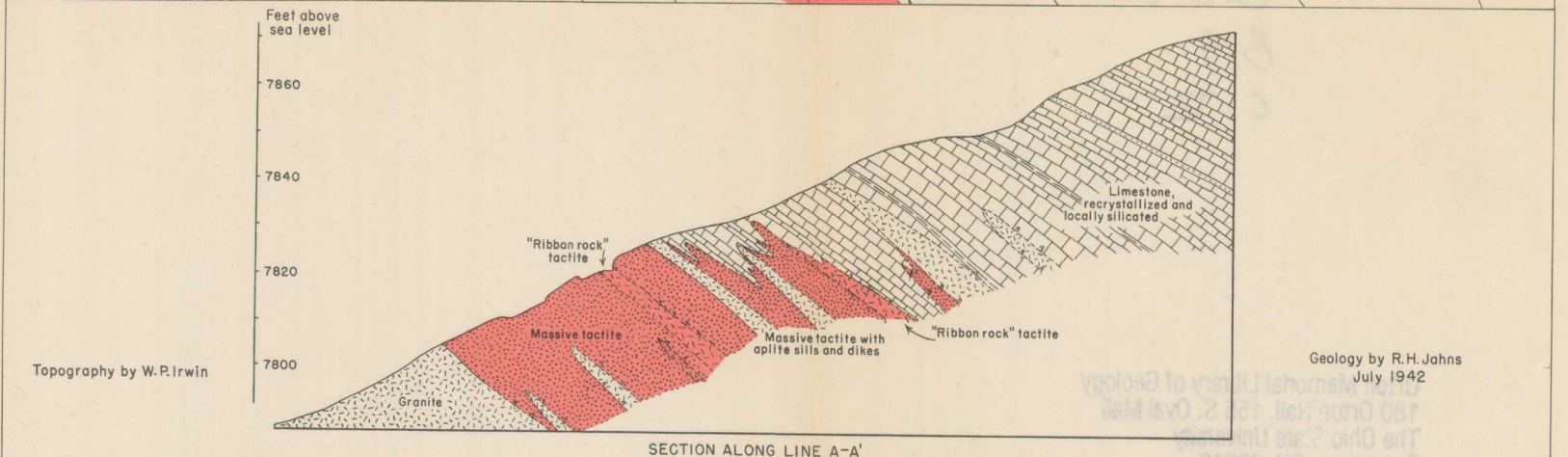
GEOLOGIC MAP AND SECTION OF THE BROWN AREA, IRON MOUNTAIN, SIERRA COUNTY, NEW MEXICO
