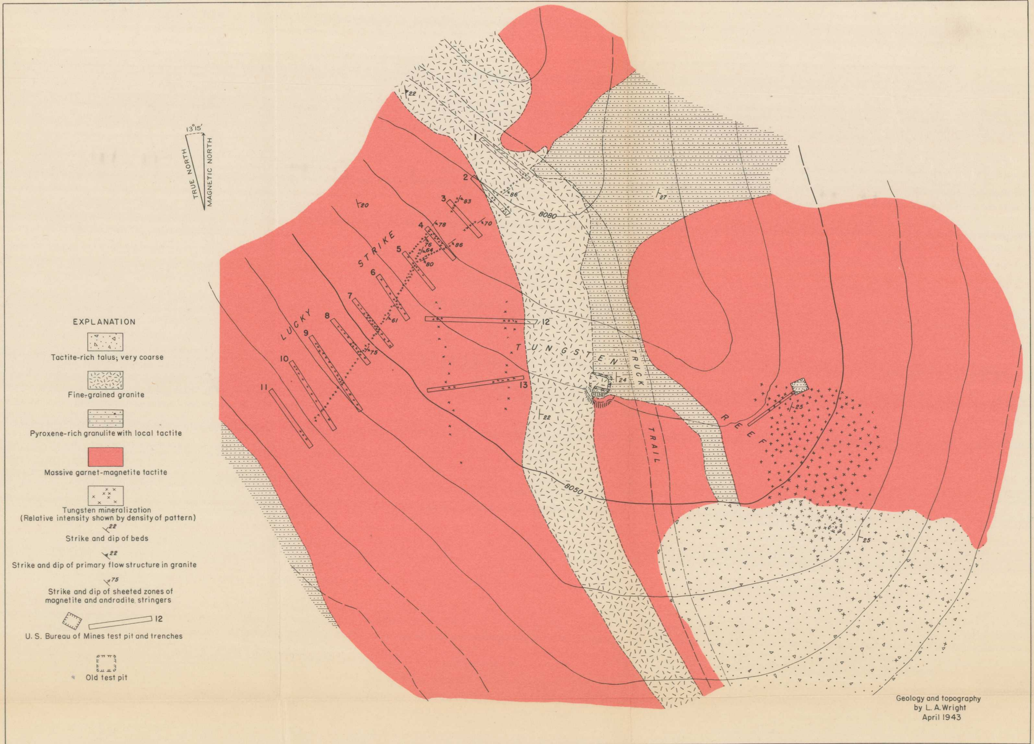
GEOLOGIC MAP OF THE LUCKY STRIKE AND TUNGSTEN REEF AREAS, IRON MOUNTAIN, SIERRA COUNTY, NEW MEXICO
