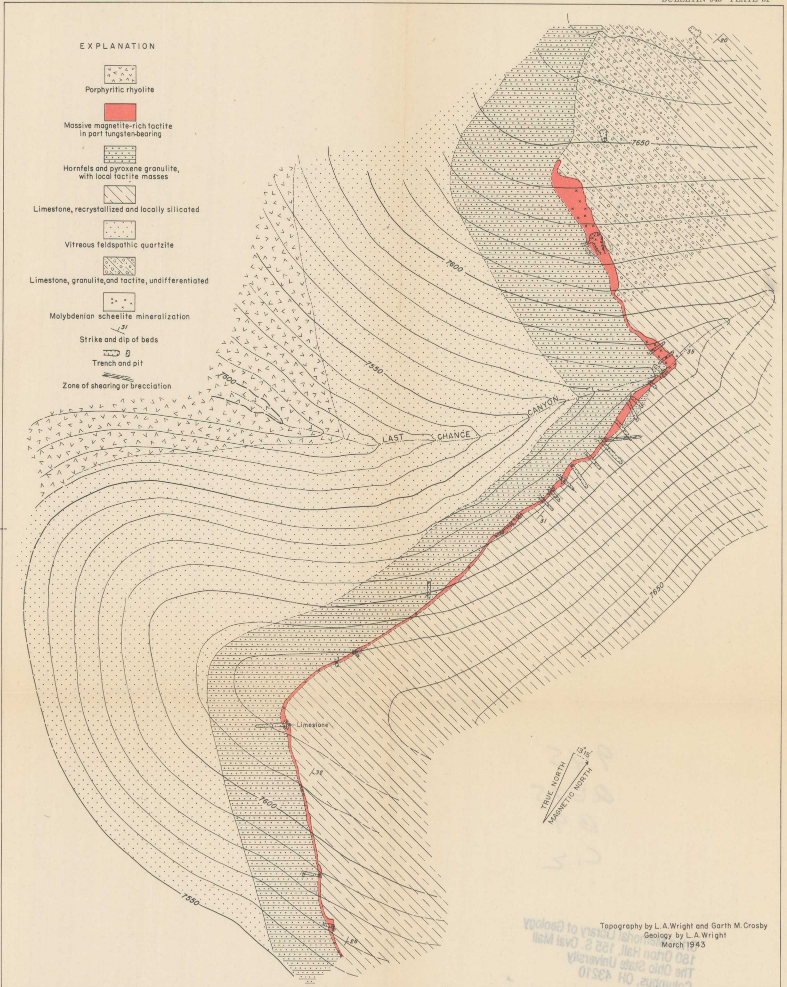
GEOLOGIC MAP OF THE BLACK BED TUNGSTEN AREA, IRON MOUNTAIN, SIERRA COUNTY, NEW MEXICO
