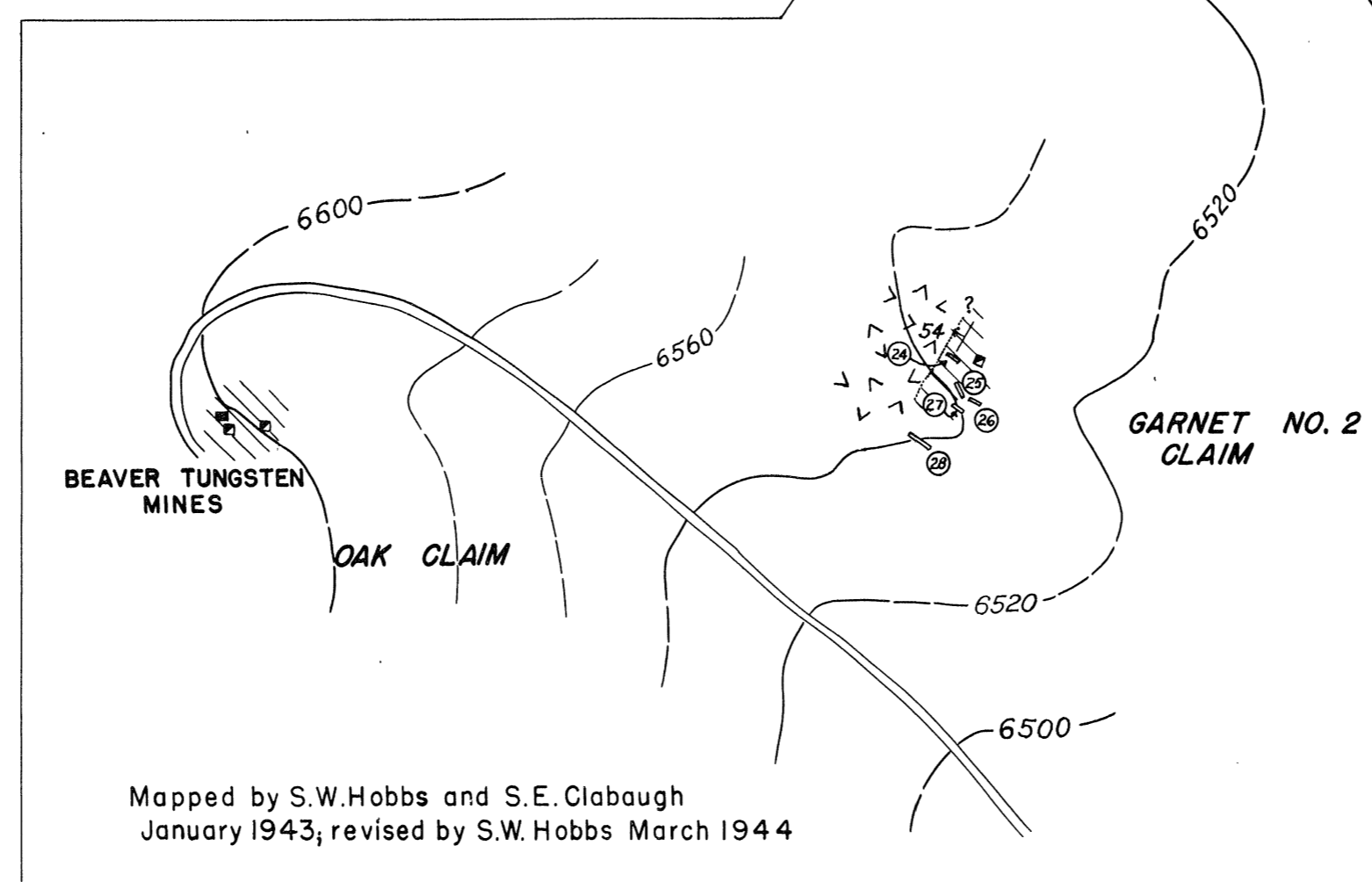
GEOLOGIC MAP OF THE SURFACE
