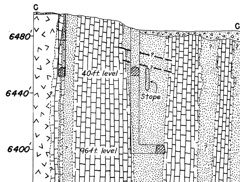
SECTION C-C'
