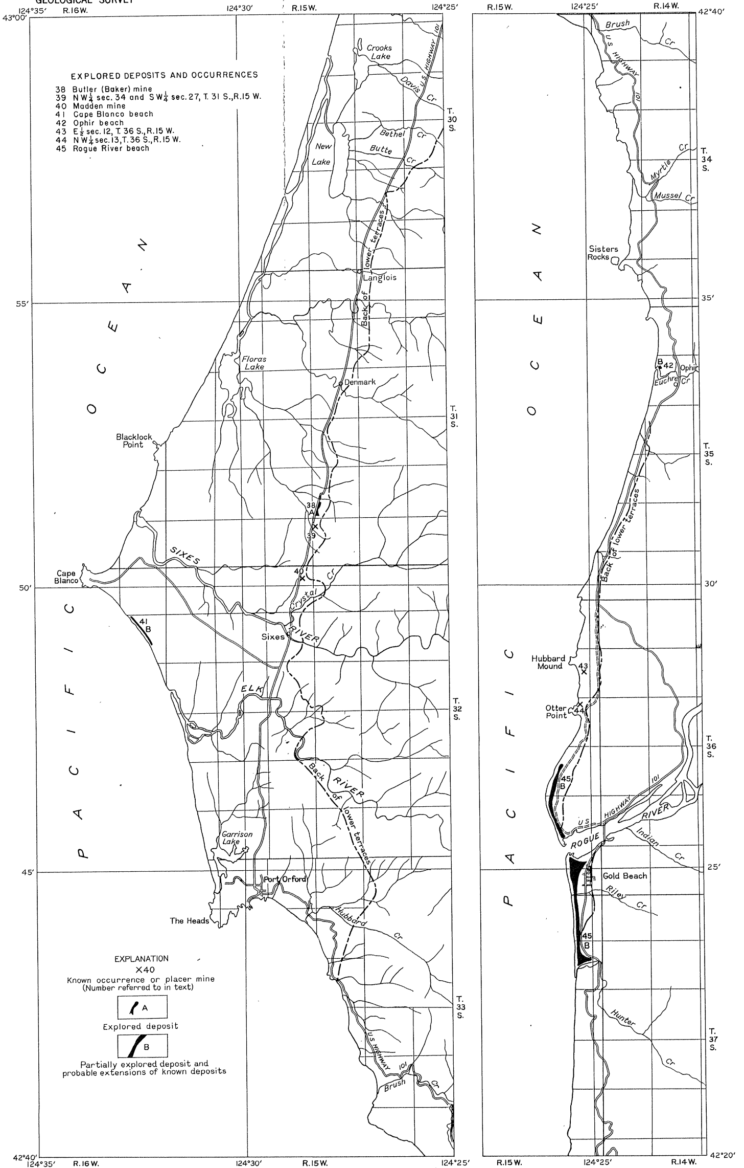
MAP OF THE SOUTHWEST COAST OF OREGON BETWEEN THE 42° 20' AND 43° PARALLELS, SHOWING DISTRIBUTION OF CHROMIFEROUS SANDS AND UPPER LIMIT OF LOWER COASTAL TERRACES
