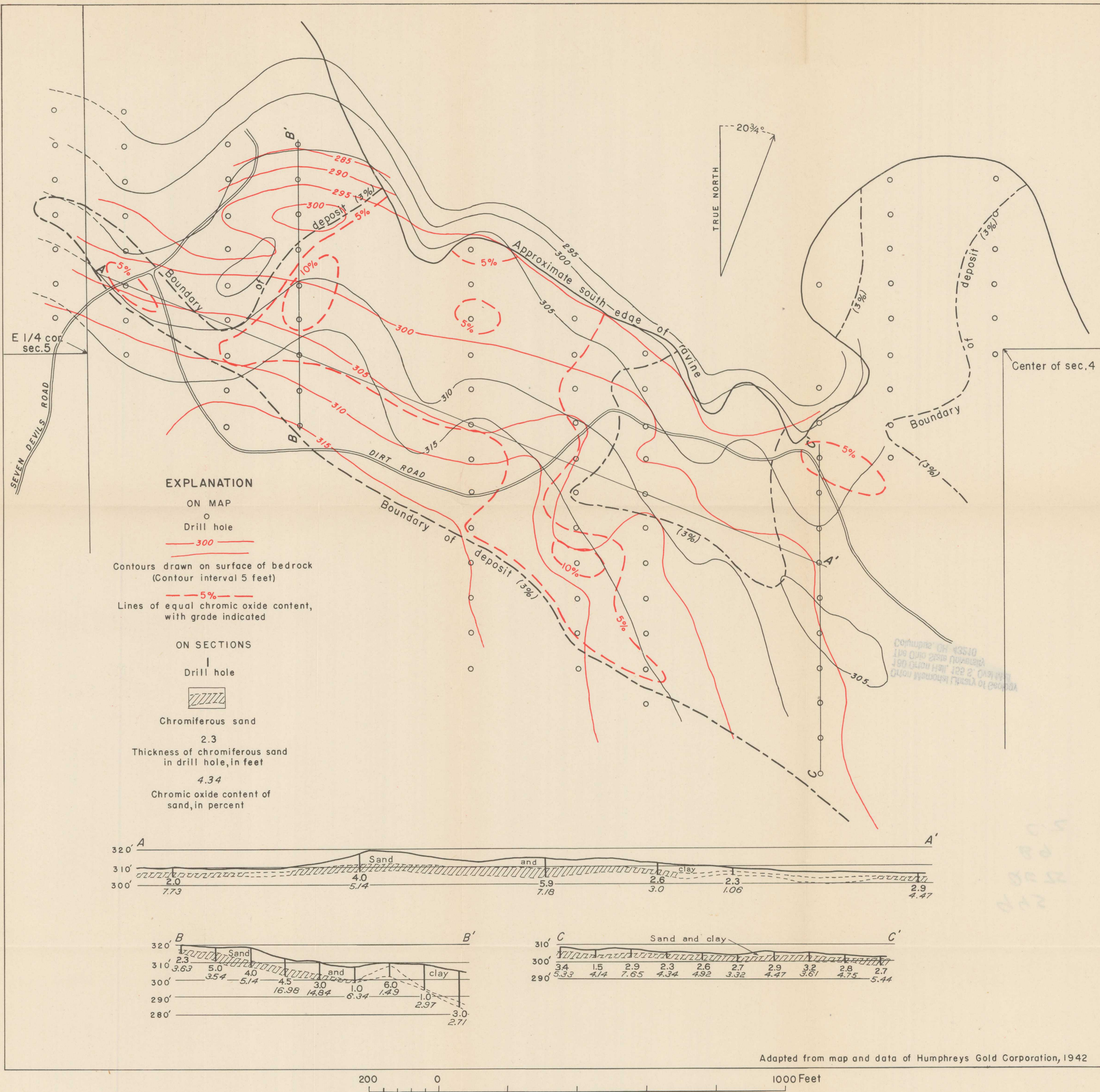
MAP AND SECTIONS OF THE SECTION 4 DEPOSIT, SHOWING RELATION BETWEEN CHROMITE CONTENT AND CONFIGURATION OF BEDROCK SURFACE
