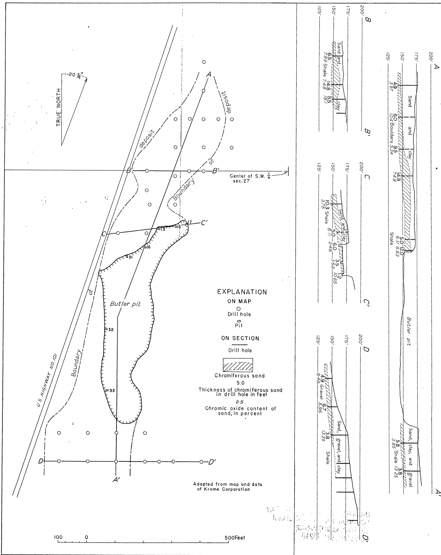
MAP AND SECTIONS OF THE BUTLER (BAKER) MINE
