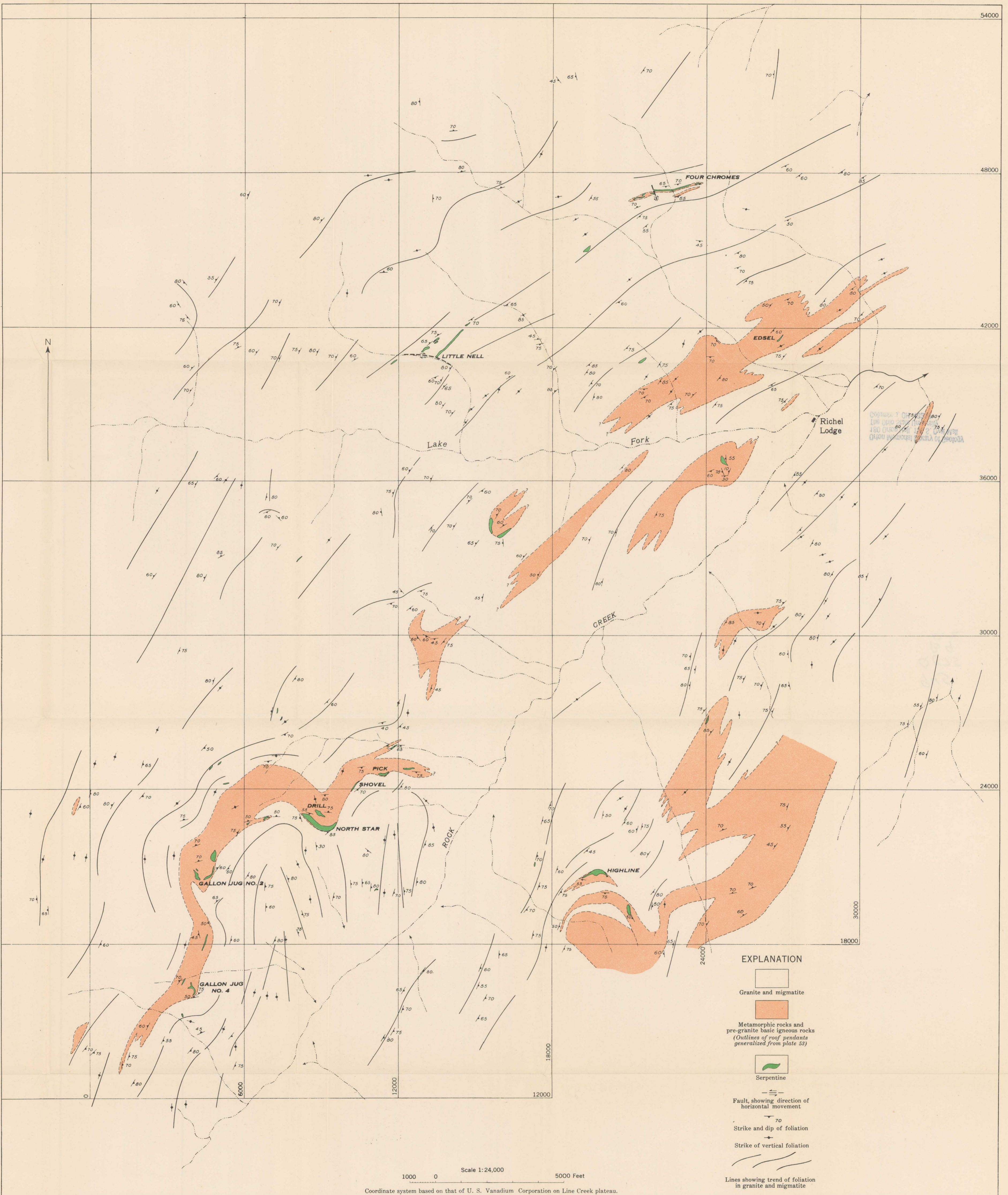
STRUCTURAL MAP OF THE RED LODGE CHROMITE AREA, CARBON COUNTY, MONTANA
