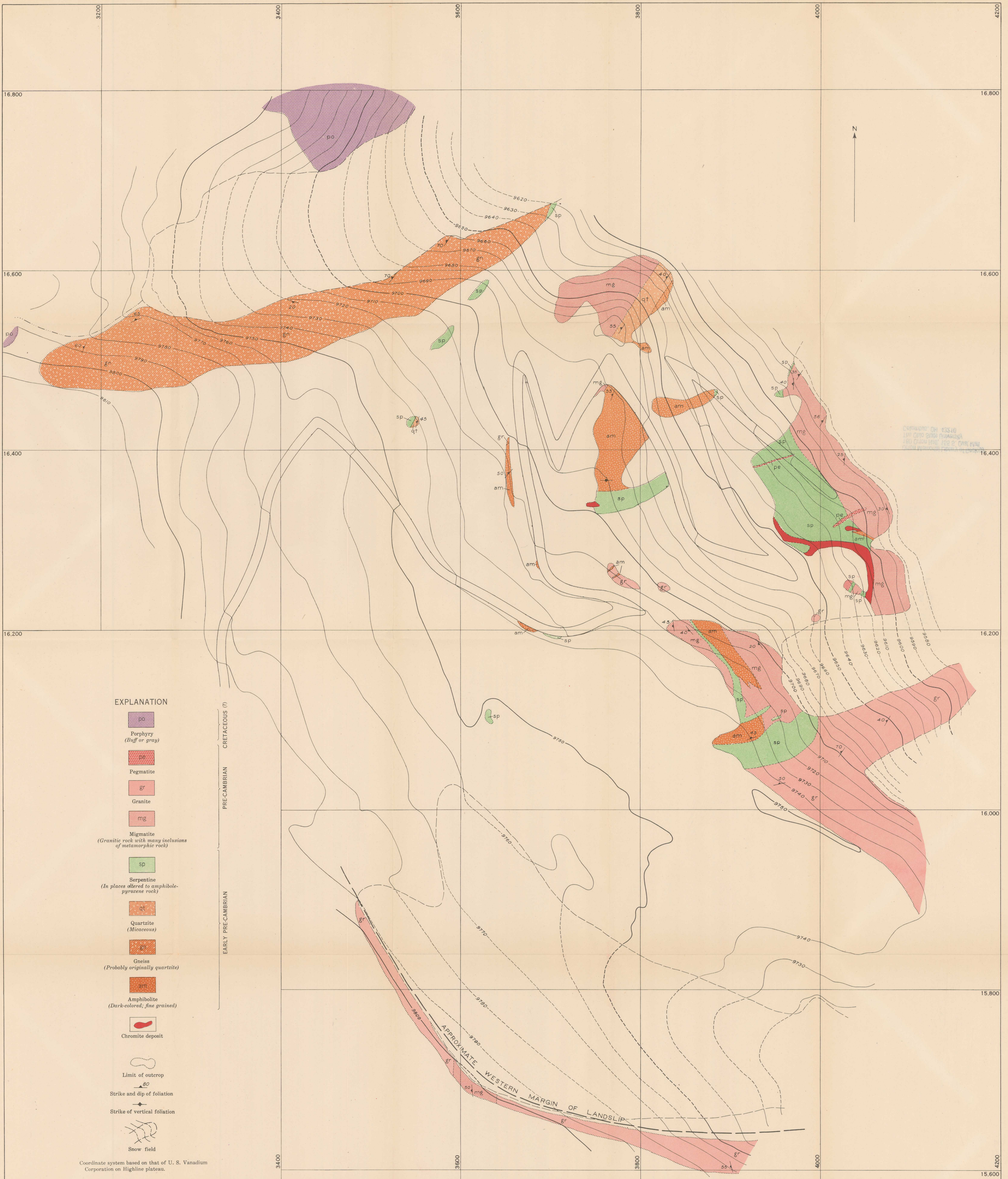
GEOLOGIC MAP OF THE CHROMITE DEPOSITS ON THE GALLON JUG NO. 4 CLAIM, CARBON COUNTY, MONTANA
