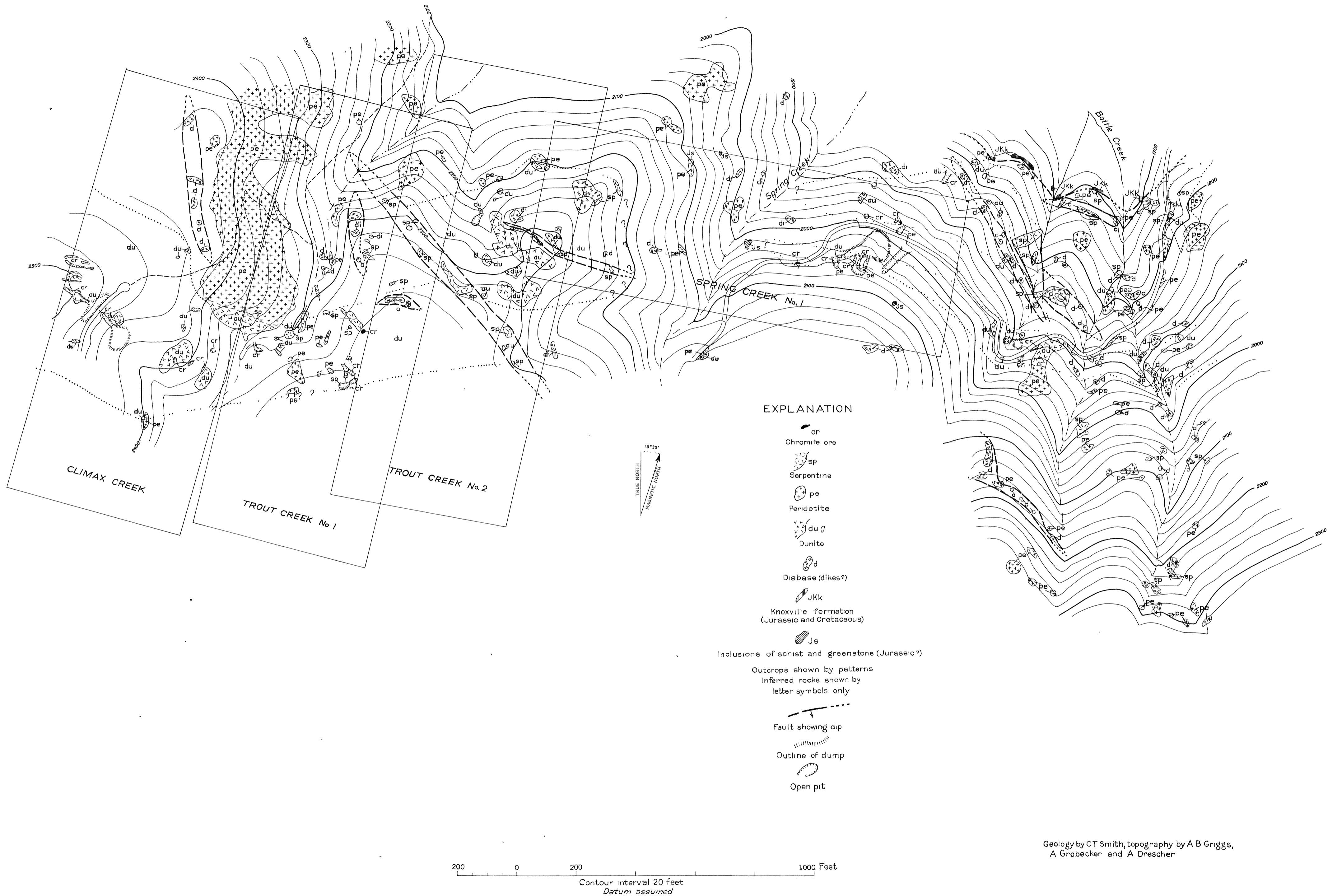
GEOLOGIC MAP OF THE CENTRAL GROUP OF THE SEELY CLAIMS, SAN LUIS OBISPO COUNTY, CALIF.
