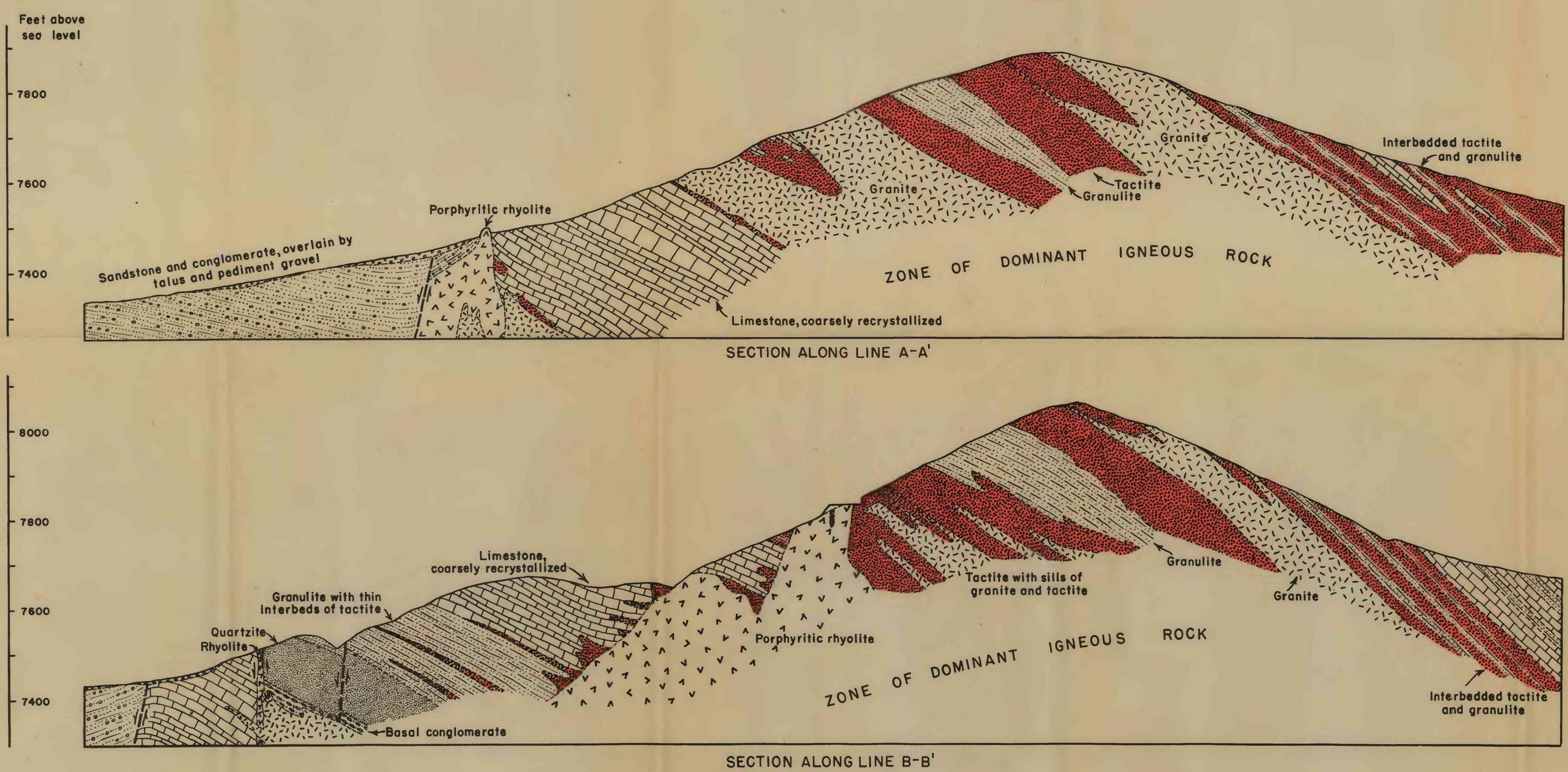
GEOLOGIC MAP AND SECTIONS OF IRON MOUNTAIN, SIERRA AND SOCORRO COUNTIES, NEW MEXICO
