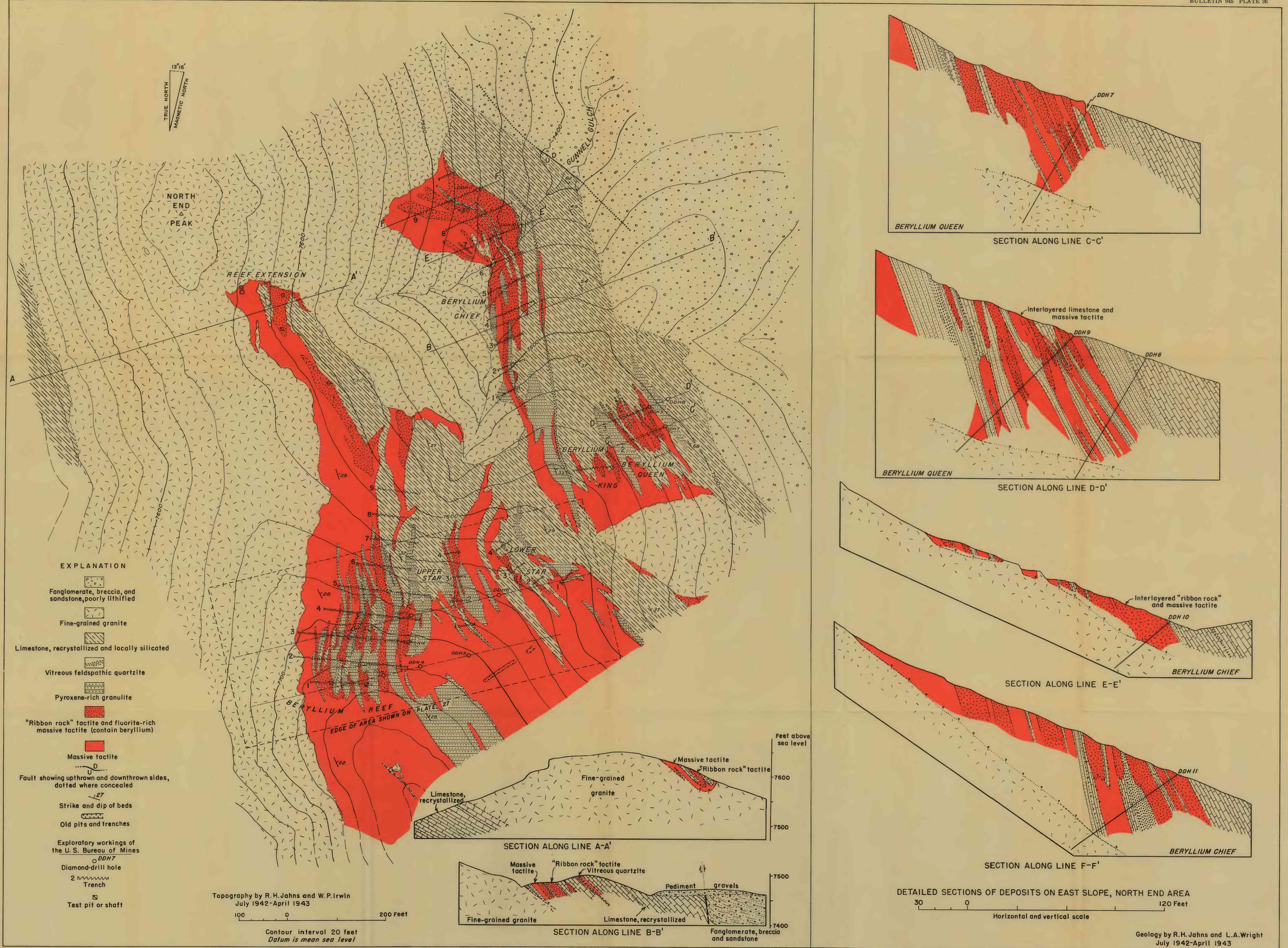
GEOLOGIC MAP AND SECTIONS OF THE NORTH END AREA, IRON MOUNTAIN, SOCORRO COUNTY, NEW MEXICO
