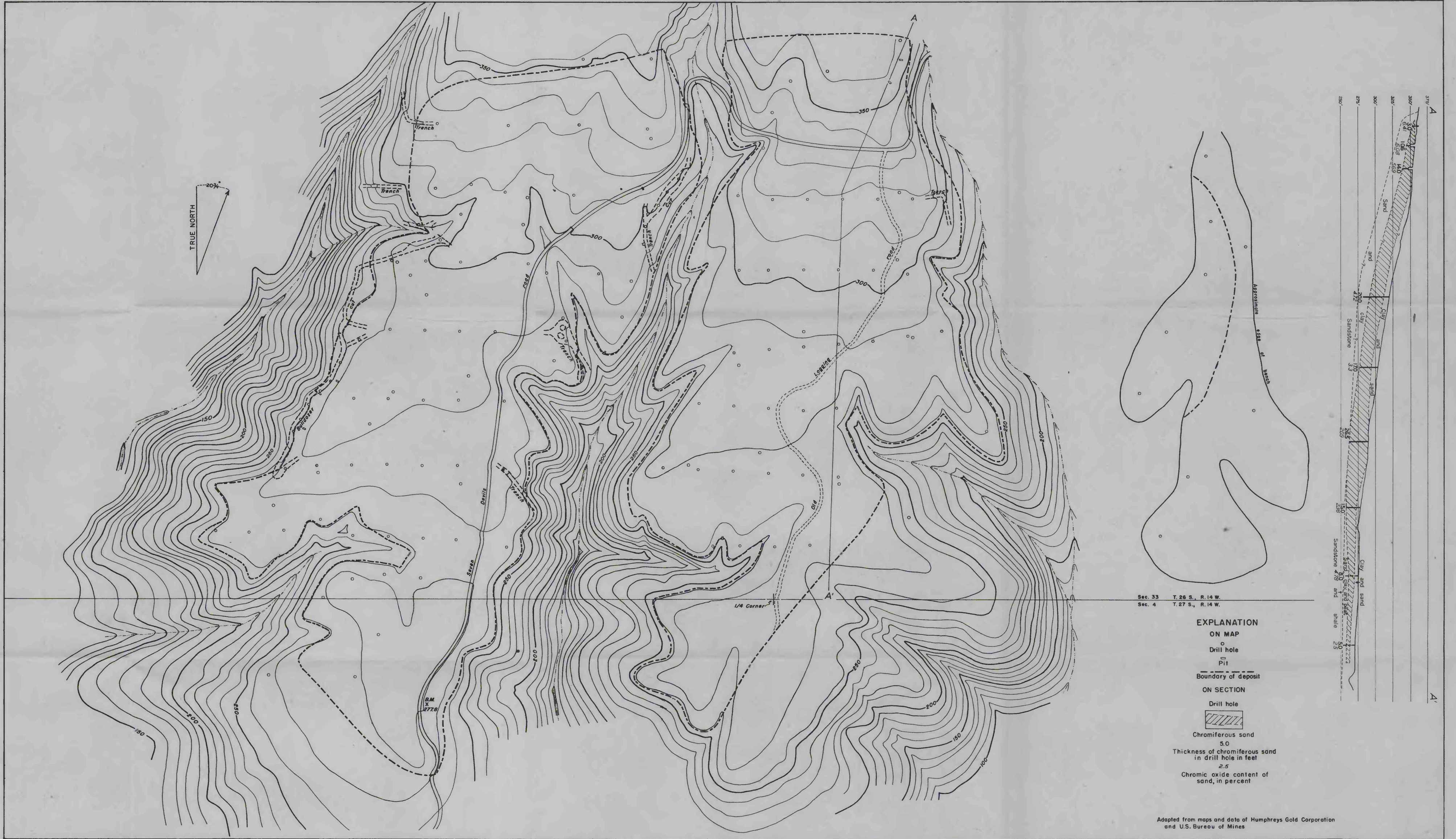
EXPLORATION MAP AND SECTION OF SECTION 33 CHROMIFEROUS SAND DEPOSIT, COOS COUNTY, OREGON
