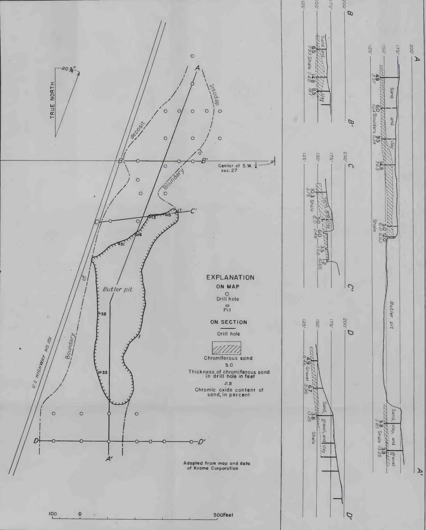
MAP AND SECTIONS OF THE BUTLER (BAKER) MINE
