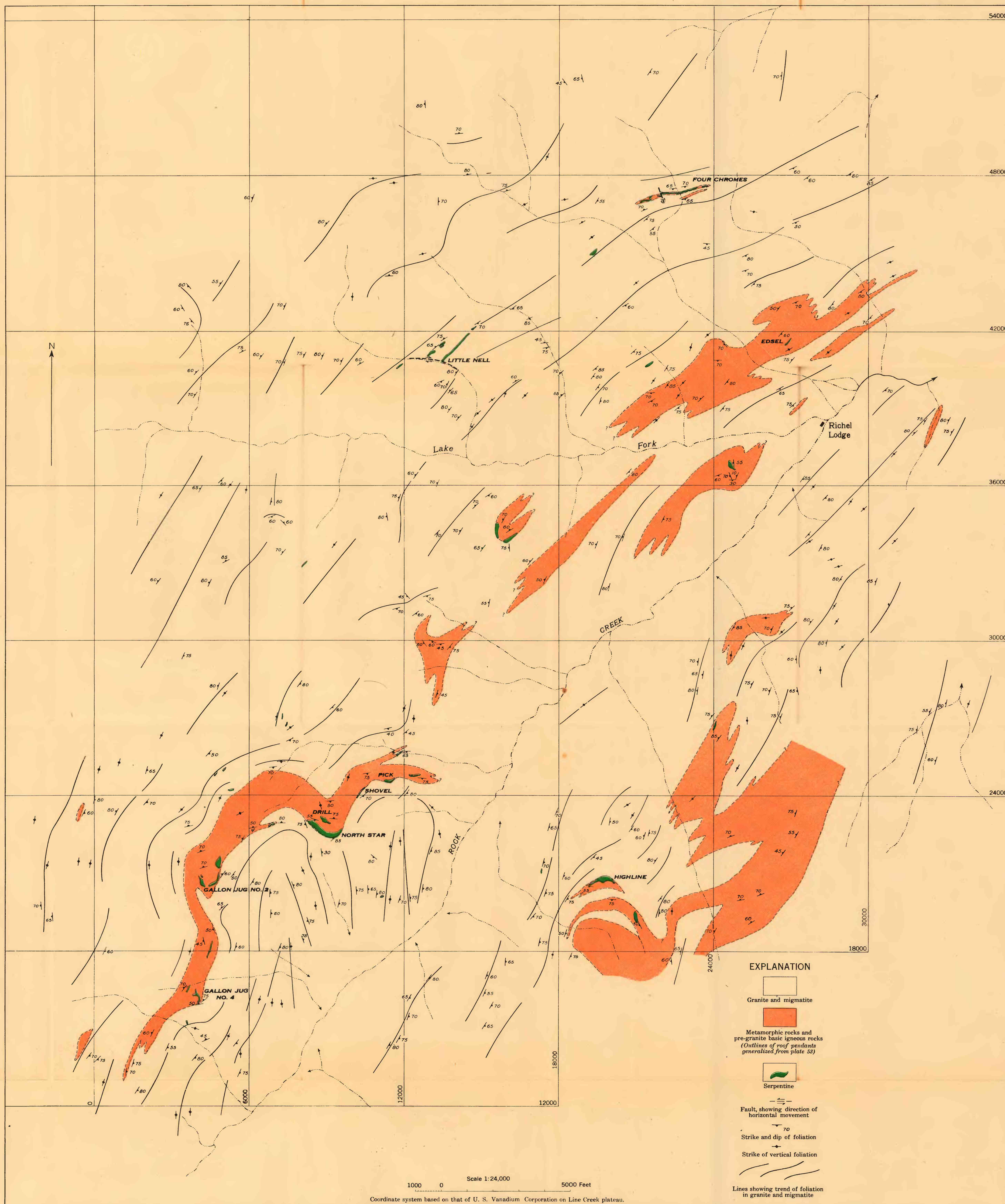
STRUCTURAL MAP OF THE RED LODGE CHROMITE AREA, CARBON COUNTY, MONTANA
