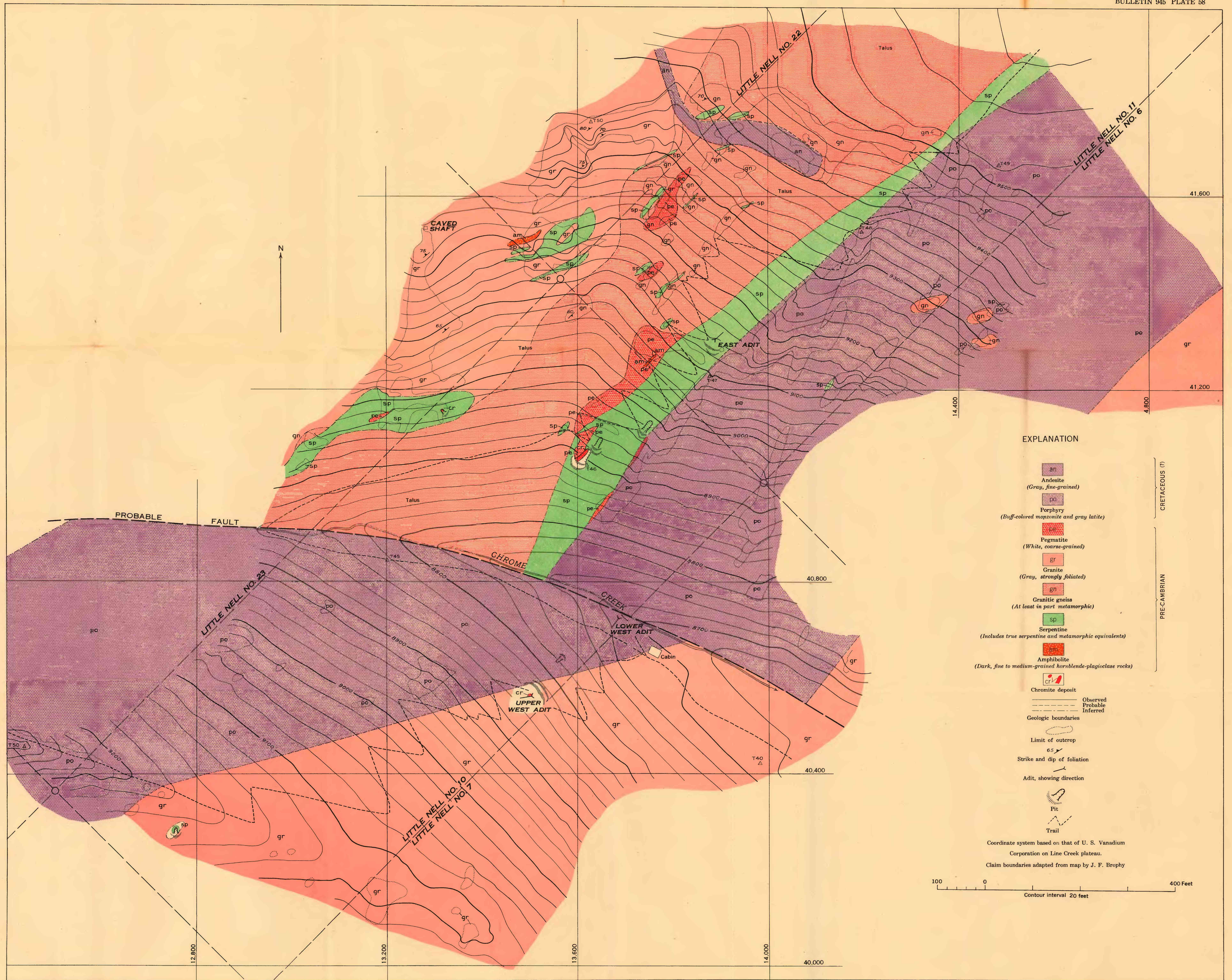
GEOLOGIC MAP OF A PART OF THE LITTLE NELL GROUP OF CLAIMS, CARBON COUNTY, MONTANA
