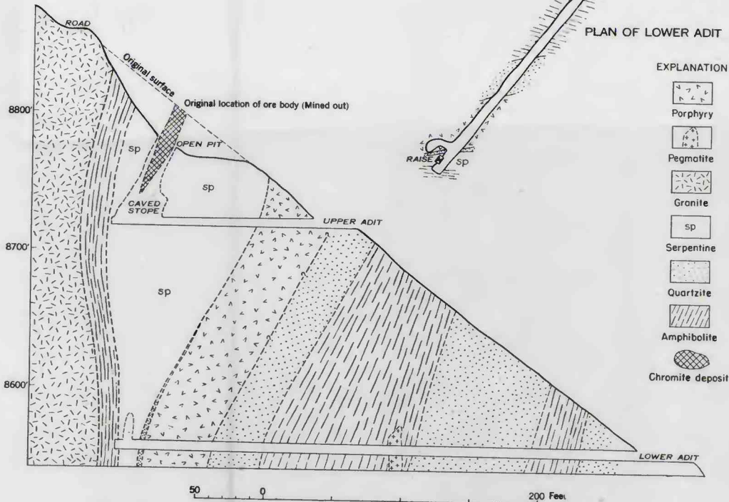
MAPS AND SECTION OF THE PICK MINE, CARBON COUNTY, MONTANA
