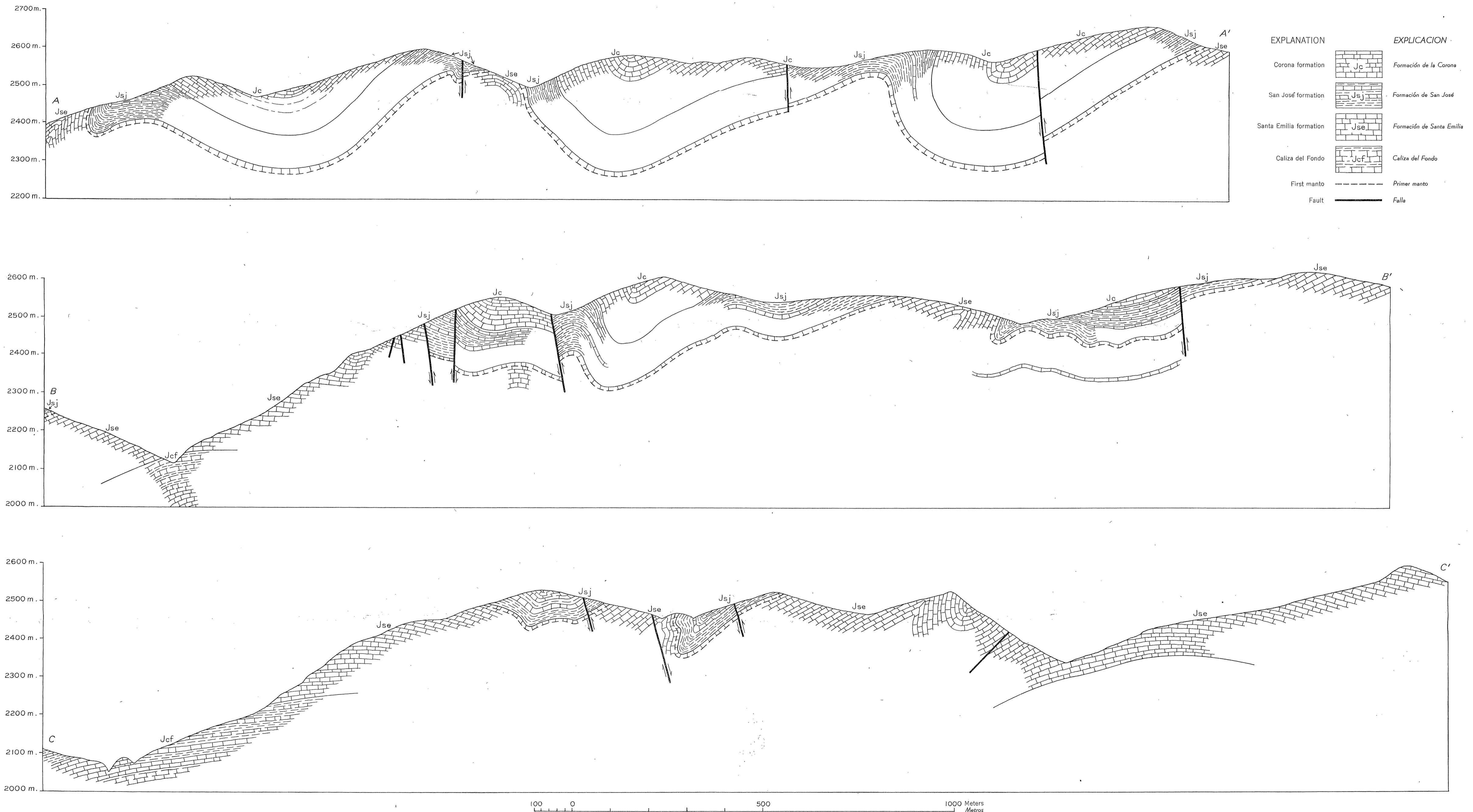
STRUCTURE SECTIONS A-A' TO C-C', OF THE SAN JOSE MINE AREA, WADLEY, STATE OF SAN LUIS POTOSI, MEXICO PERFILES A-A' HASTA C-C', DEL AREA DE LA MINA DE SAN JOSE, WADLEY, ESTADO DE SAN LUIS POTOSI, MEXICO
