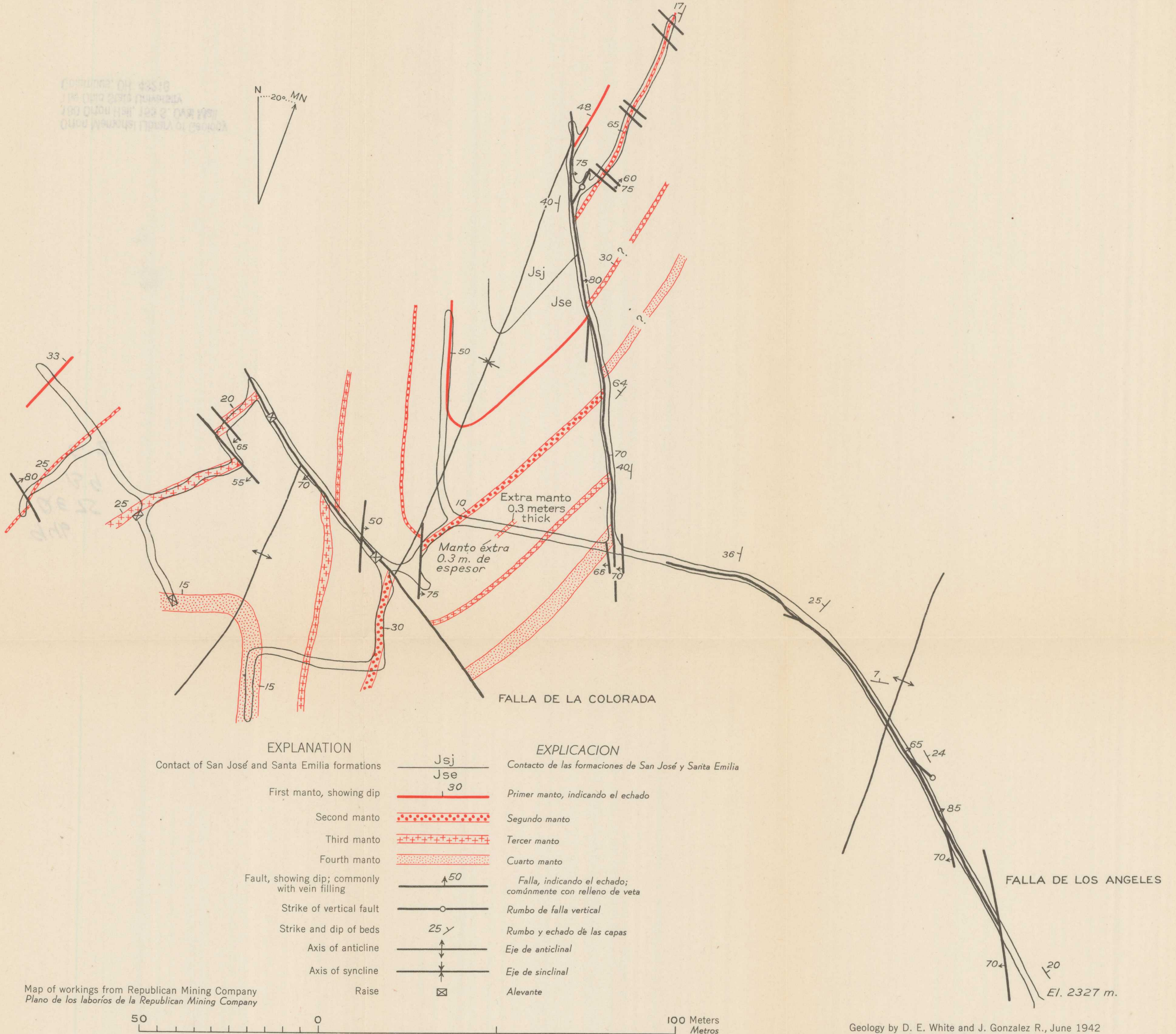
PLAN OF THE SAN FELIPE TUNNEL, SANTA EMILIA MINE, WADLEY, STATE OF SAN LUIS POTOSI, MEXICO PLANO DEL TUNEL DE SAN FELIPE, MINA DE SANTA EMILIA, WADLEY, ESTADO DE SAN LUIS POTOSI, MEXICO
