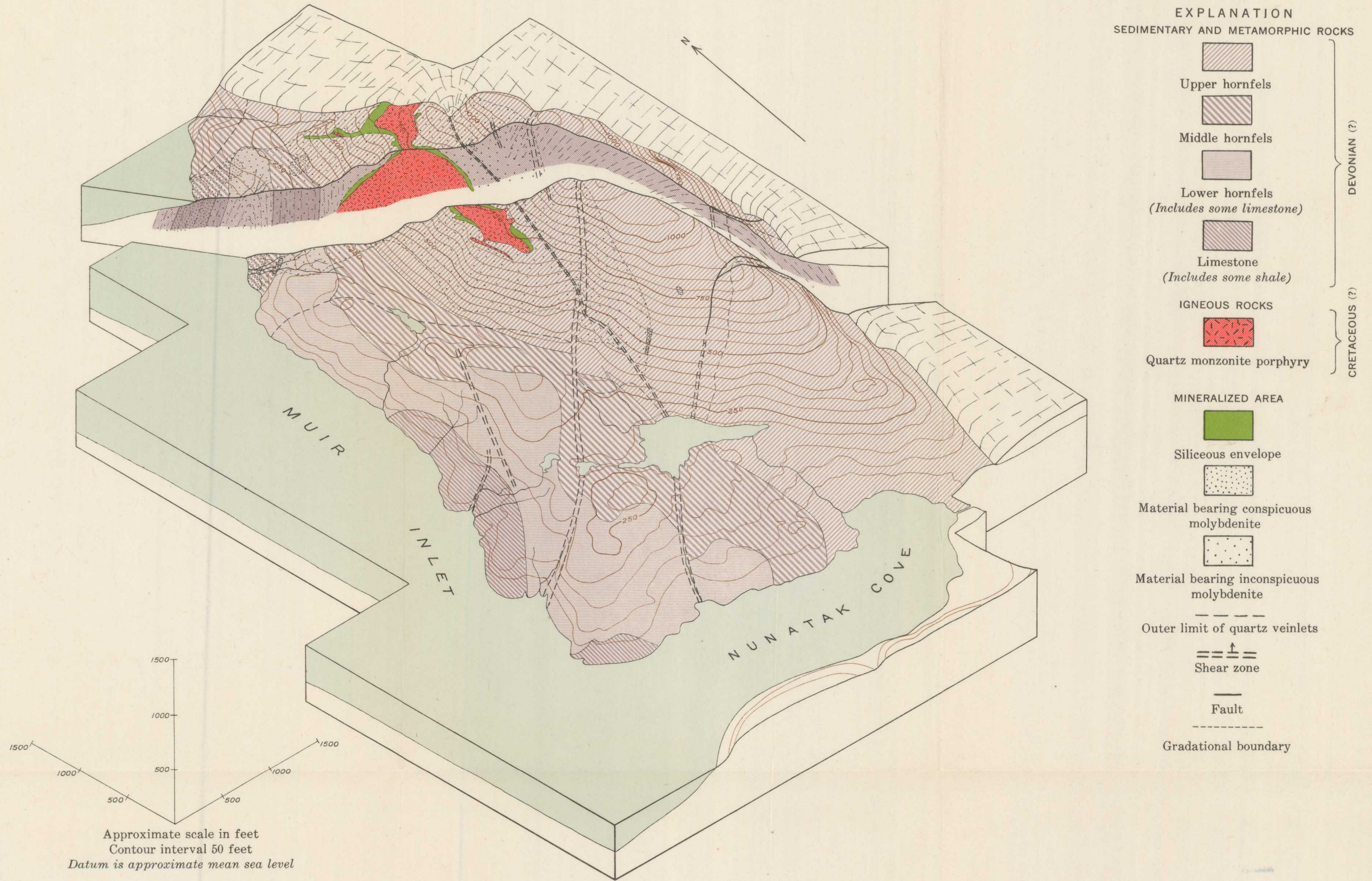
GEOLOGIC ISOMETRIC BLOCK DIAGRAM OF NUNATAK AREA, MUIR INLET, GLACIER BAY, SOUTHEASTERN ALASKA
