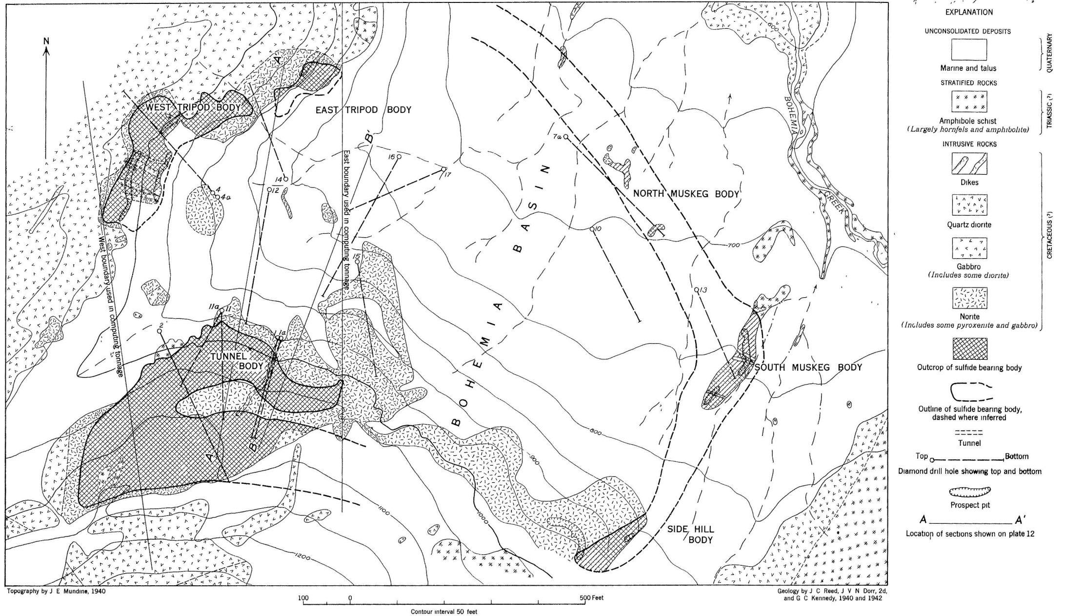
GEOLOGIC MAP SHOWING LOCATION OF DRILL HOLES IN AND NEAR THE TRIPOD, TUNNEL, SIDE HILLS, AND MUSKEG SULFIDE-BEARING BODIES, SOUTHEASTERN ALASKA
