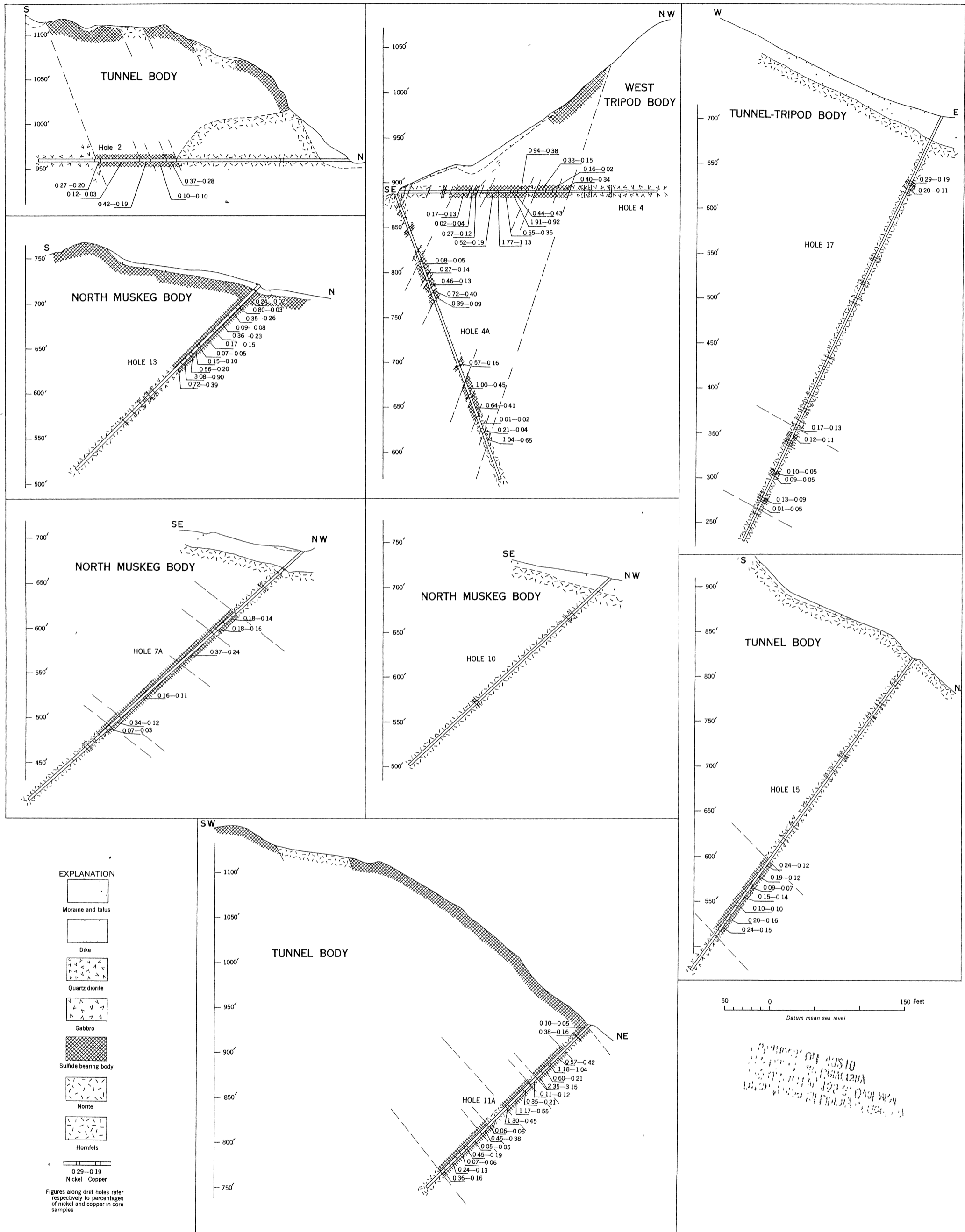
SECTIONS THROUGH CERTAIN DRILL HOLES IN THE TUNNEL, TRIPOD, AND MUSKEG SULFIDE-BEARING BODIES, SOUTHEASTERN ALASKA
