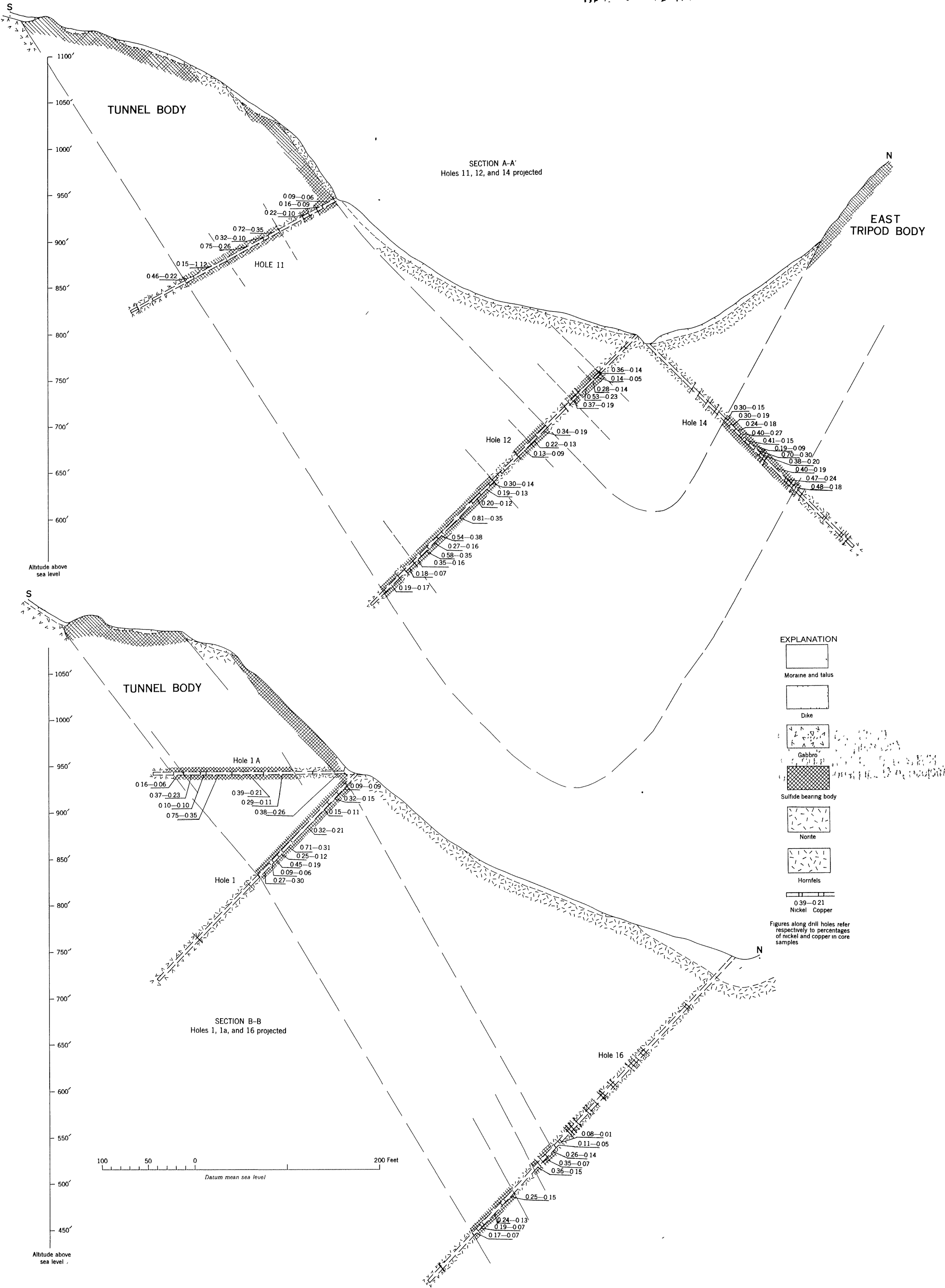
GEOLOGIC SECTIONS ACROSS SULFIDE-BEARING DEPOSITS, YAKOBI ISLAND SOUTHEASTERN ALASKA
