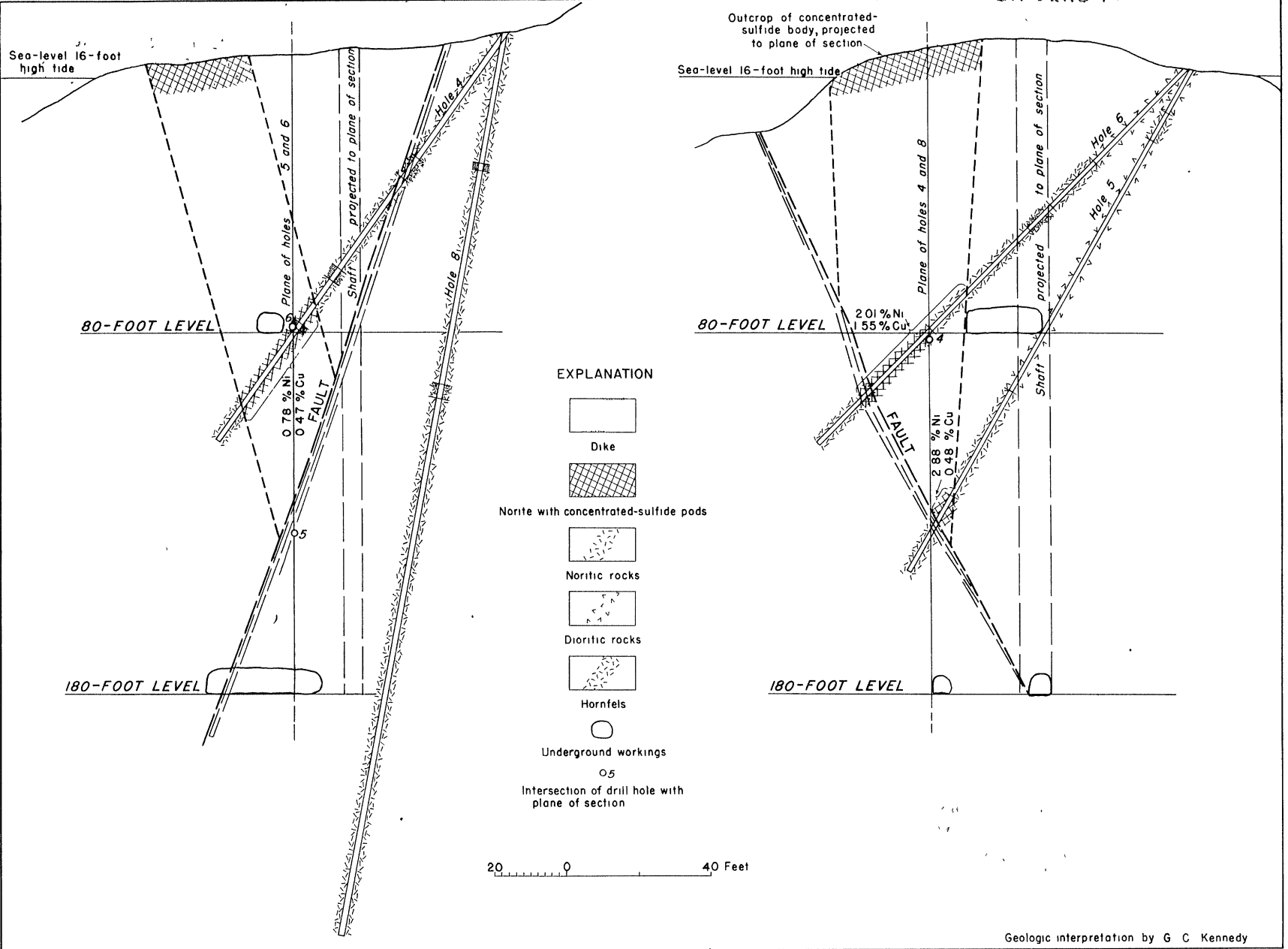
CROSS SECTIONS OF CONCENTRATED-SULFIDE DEPOSIT ON FLEMING ISLAND, SOUTHEASTERN ALASKA
