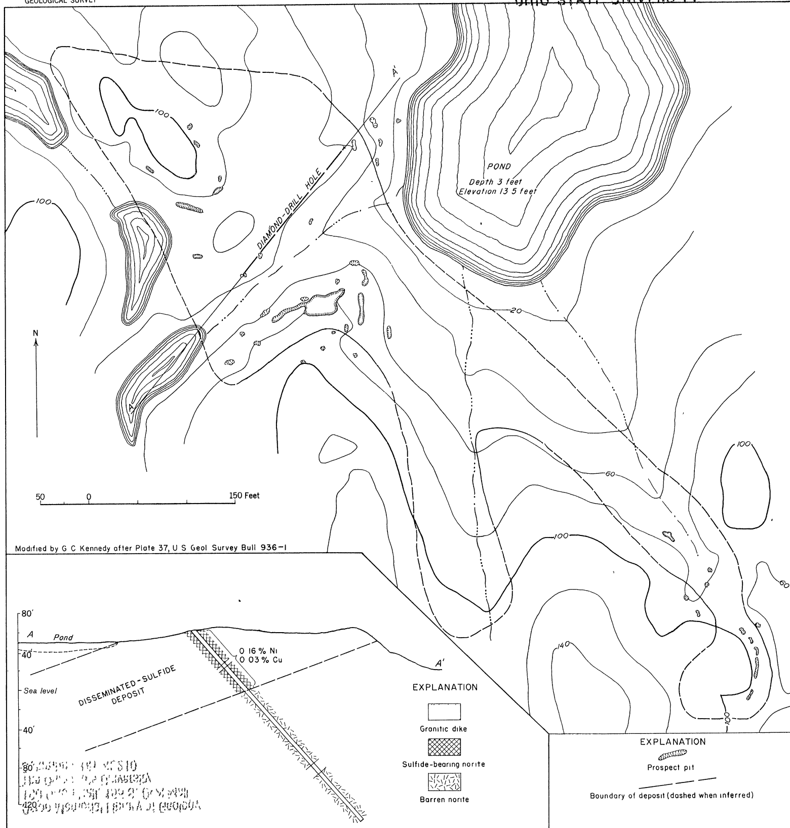
MAP AND CROSS SECTION OF DISSEMINATED-SULFIDE DEPOSIT ON CHICHAGOF ISLAND, SOUTHEASTERN ALASKA
